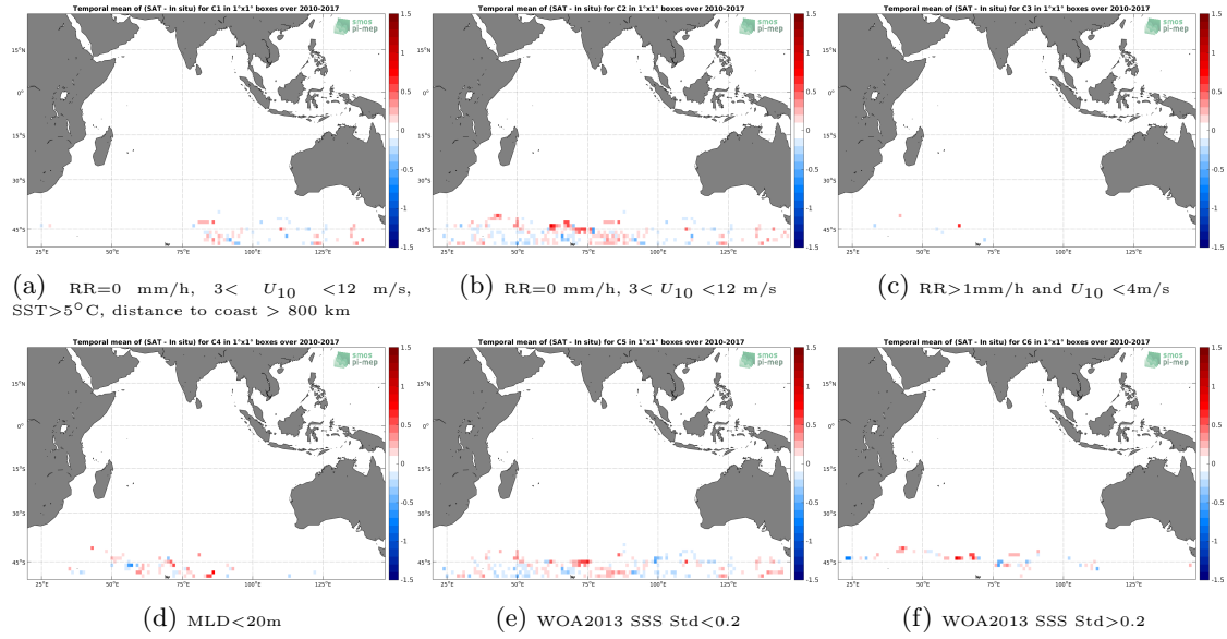
Figure 12: Temporal mean gridded over spatial boxes of size 1^{\circ}\times 1^{\circ} of \Delta\text{SSS} (CCI L4 Merged-OI v2.31 - 30-day running (ESA) - Sea mammals) for 6 different subdatasets corresponding to: \text{RR}=0 mm/h, 3 < U_{10} < 12 m/s, SST > 5^{\circ}\text{C} , distance to coast > 800 km (a), \text{RR}=0 mm/h, 3 < U_{10} < 12 m/s (b), \text{RR} > 1\text{mm/h} and U_{10} < 4\text{m/s} (c), \text{MLD} < 20\text{m} (d), WOA2013 SSS Std < 0.2 (e), WOA2013 SSS Std > 0.2 (f).
