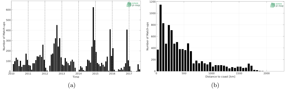
Figure 1: Number of match-ups between Sea mammals and CCI L4 Merged-OI v2.31 - 30-day running (ESA) SSS as a function of time (a) and as function of the distance to coast (b) over the Indian Ocean Pi-MEP region and for the full satellite product period.
