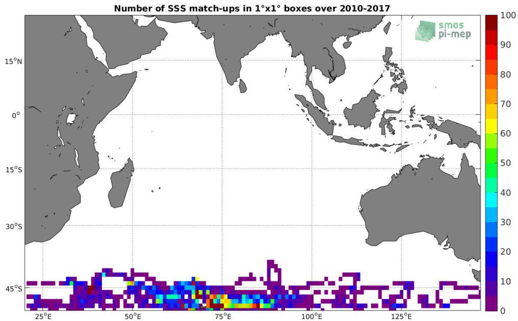
Figure 4: Number of SSS match-ups between Sea mammals SSS and the CCI L4 Merged-OI v2.31 - 30-day running (ESA) SSS product for the Indian Ocean Pi-MEP region over 1°x1° boxes and for the full satellite product period.
