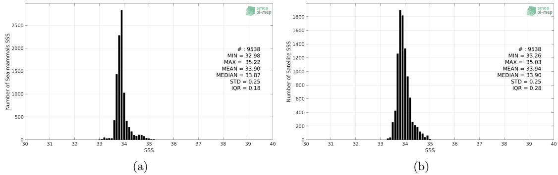
Figure 2: Histograms of SSS from Sea mammals (a) and CCI L4 Merged-OI v2.31 - 30-day running (ESA) (b) considering all match-up pairs per bins of 0.1 over the Indian Ocean Pi-MEP region and for the full satellite product period.
