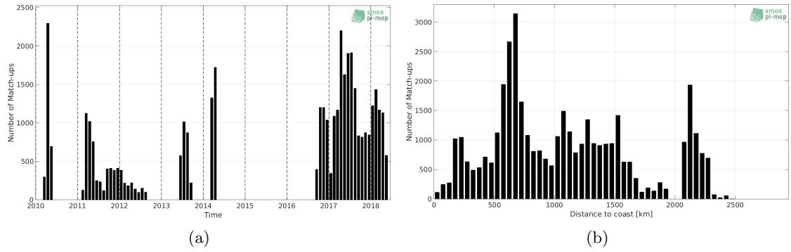
Figure 1: Number of match-ups between Surface drifters and CCI SSS L4 Merged-OI v2.31 - 30-day running (ESA) SSS as a function of time (a) and as function of the distance to coast (b) over the Indian Ocean Pi-MEP region and for the full satellite product period.
