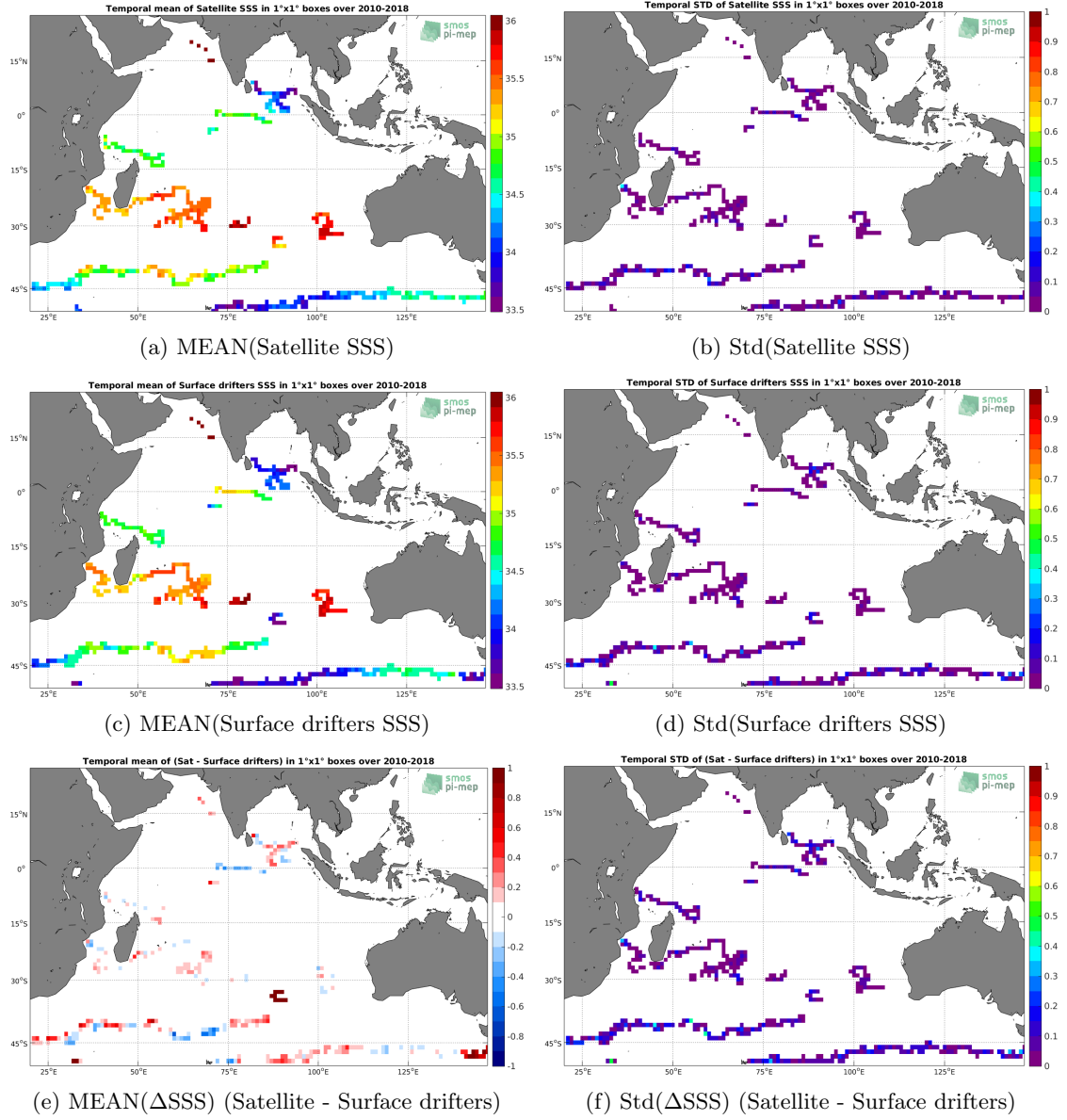
Figure 5: Temporal mean (left) and Std (right) of SSS from CCI SSS L4 Merged-OI v2.31 - 30-day running (ESA) (top), Surface drifters (middle), and of \Delta SSS (Satellite - Surface drifters). Only match-up pairs are used to generate these maps.
