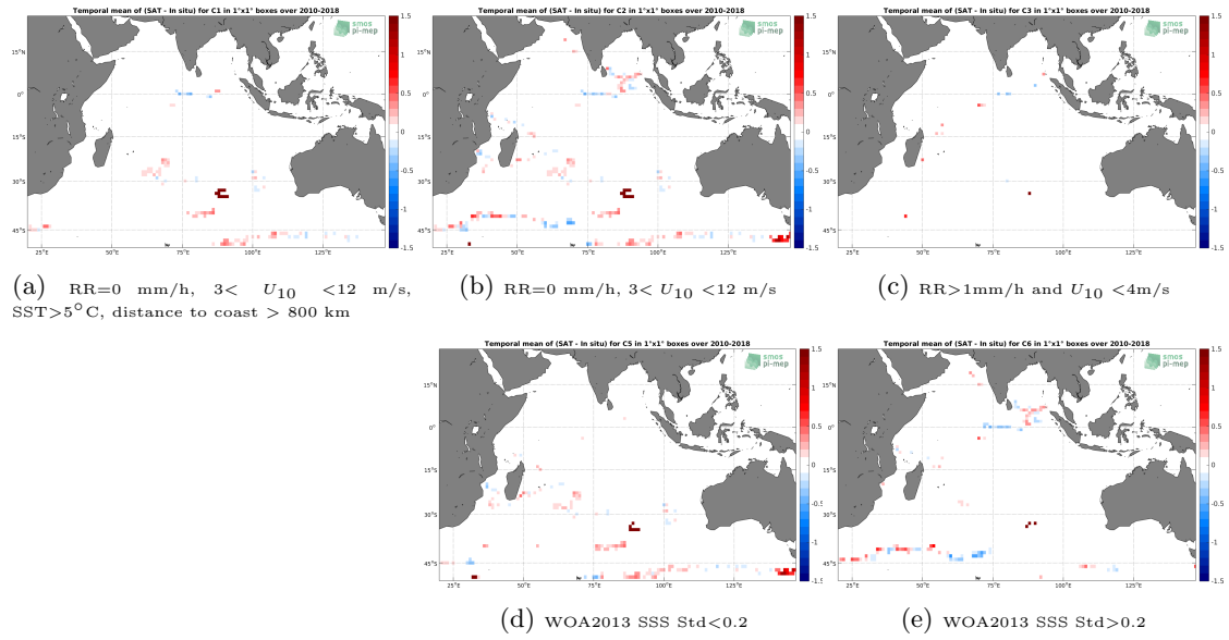
Figure 11: Temporal mean gridded over spatial boxes of size 1^\circ \times 1^\circ of \Delta SSS (CCI SSS L4 Merged-OI v2.31 - 30-day running (ESA) - Surface drifters) for 5 different subdatasets corresponding to: RR=0 mm/h, 3 < U_{10} < 12 m/s, SST >5^\circ C, distance to coast > 800 km (a), RR=0 mm/h, 3 < U_{10} < 12 m/s (b), RR >1 mm/h and U_{10} < 4 m/s (c), WOA2013 SSS Std <0.2 (d), WOA2013 SSS Std >0.2 (e).
