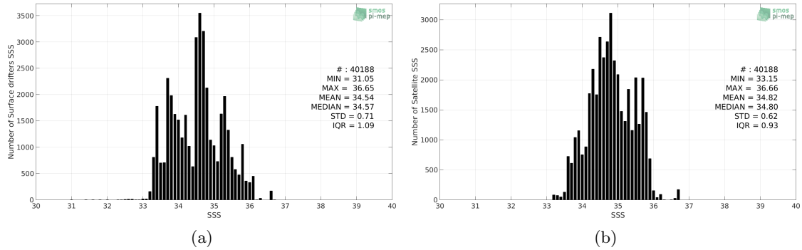
Figure 2: Histograms of SSS from Surface drifters (a) and CCI SSS L4 Merged-OI v2.31 - 30-day running (ESA) (b) considering all match-up pairs per bins of 0.1 over the Indian Ocean Pi-MEP region and for the full satellite product period.
