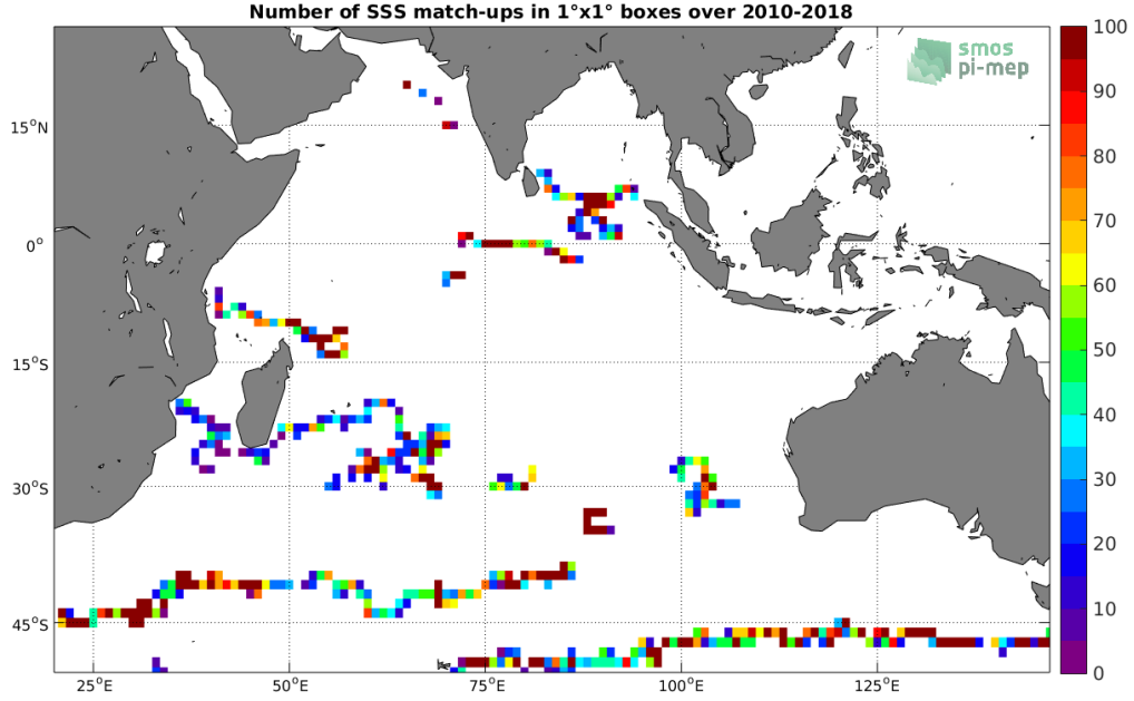
Figure 3: Number of SSS match-ups between Surface drifters SSS and the CCI SSS L4 Merged-OI v2.31 - 30-day running (ESA) SSS product for the Indian Ocean Pi-MEP region over 1^\circ \times 1^\circ boxes and for the full satellite product period.
