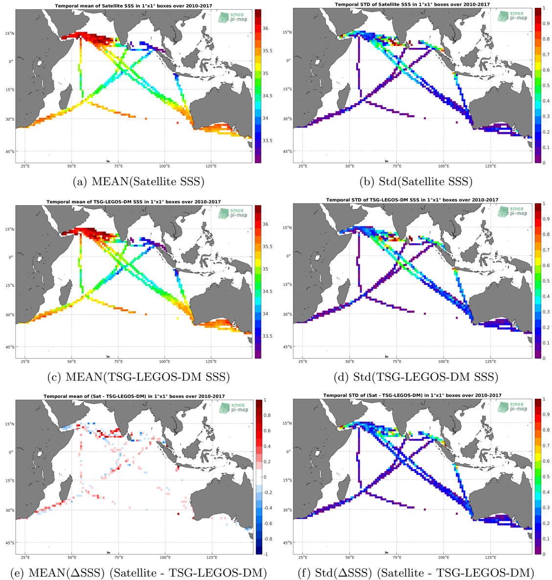
Figure 6: Temporal mean (left) and Std (right) of SSS from CCI L4 Merged-OI v1.8 - 7-day running (ESA) (top), TSG-LEGOS-DM (middle), and of \Delta SSS (Satellite - TSG-LEGOS-DM). Only match-up pairs are used to generate these maps.
