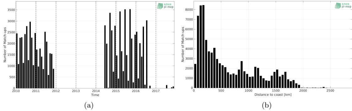
Figure 1: Number of match-ups between TSG-LEGOS-DM and CCI L4 Merged-OI v1.8 - 7-day running (ESA) SSS as a function of time (a) and as function of the distance to coast (b) over the Indian Ocean Pi-MEP region and for the full satellite product period.
