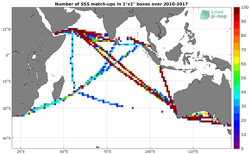
Figure 4: Number of SSS match-ups between TSG-LEGOS-DM SSS and the CCI L4 Merged-OI v1.8 - 7-day running (ESA) SSS product for the Indian Ocean Pi-MEP region over 1°x1° boxes and for the full satellite product period.
