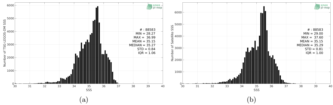
Figure 2: Histograms of SSS from TSG-LEGOS-DM (a) and CCI L4 Merged-OI v1.8 - 7-day running (ESA) (b) considering all match-up pairs per bins of 0.1 over the Indian Ocean Pi-MEP region and for the full satellite product period.
