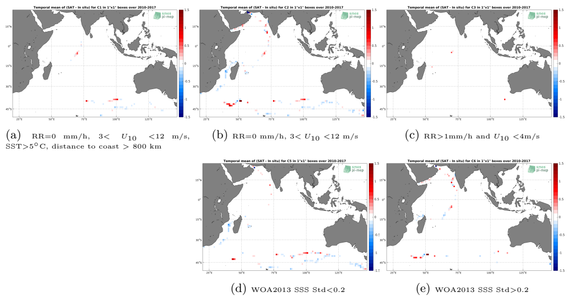
Figure 12: Temporal mean gridded over spatial boxes of size 1^\circ \times 1^\circ of \Delta SSS (CCI L4 Merged-OI v1.8 - 7-day running (ESA) - TSG-GOSUD-Sailing-ship) for 5 different subdatasets corresponding to: RR=0 mm/h, 3 < U_{10} < 12 m/s, SST > 5°C, distance to coast > 800 km (a), RR=0 mm/h, 3 < U_{10} < 12 m/s (b), RR > 1mm/h and U_{10} < 4 m/s (c), WOA2013 SSS Std < 0.2 (d), WOA2013 SSS Std > 0.2 (e).
