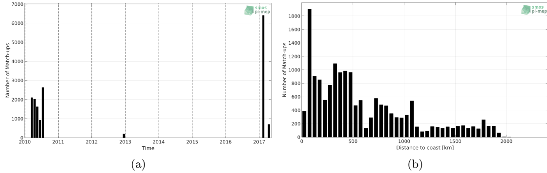
Figure 1: Number of match-ups between TSG-GOSUD-Sailing-ship and CCI L4 Merged-OI v1.8 - 7-day running (ESA) SSS as a function of time (a) and as function of the distance to coast (b) over the Indian Ocean Pi-MEP region and for the full satellite product period.
