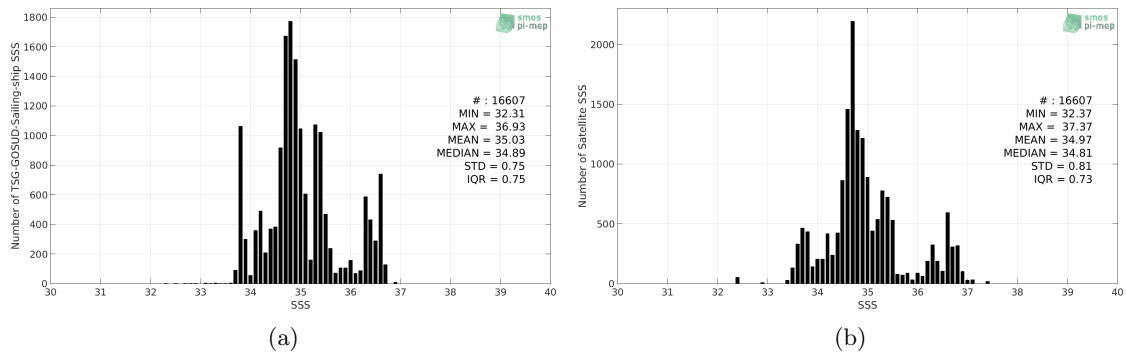
Figure 2: Histograms of SSS from TSG-GOSUD-Sailing-ship (a) and CCI L4 Merged-OI v1.8 - 7-day running (ESA) (b) considering all match-up pairs per bins of 0.1 over the Indian Ocean Pi-MEP region and for the full satellite product period.
