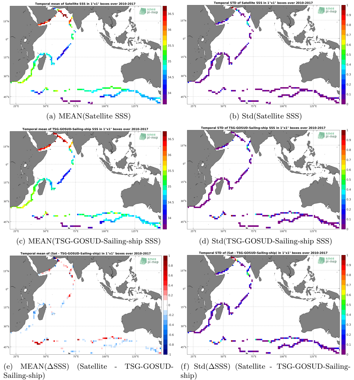
Figure 6: Temporal mean (left) and Std (right) of SSS from CCI L4 Merged-OI v1.8 - 7-day running (ESA) (top), TSG-GOSUD-Sailing-ship (middle), and of \Delta SSS (Satellite - TSG-GOSUD-Sailing-ship). Only match-up pairs are used to generate these maps.
