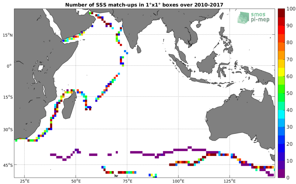
Figure 4: Number of SSS match-ups between TSG-GOSUD-Sailing-ship SSS and the CCI L4 Merged-OI v1.8 - 7-day running (ESA) SSS product for the Indian Ocean Pi-MEP region over 1°x1° boxes and for the full satellite product period.
