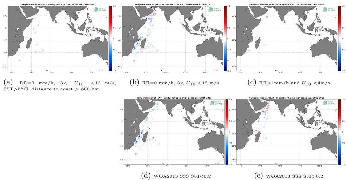
Figure 12: Temporal mean gridded over spatial boxes of size 1^\circ \times 1^\circ of \Delta SSS (CCI L4 Merged-OI v1.8 - 7-day running (ESA) - TSG-GOSUD-Research-vessel) for 5 different subdatasets corresponding to: RR=0 mm/h, 3 < U_{10} < 12 m/s, SST > 5^\circ\text{C} , distance to coast > 800 km (a), RR=0 mm/h, 3 < U_{10} < 12 m/s (b), RR > 1 mm/h and U_{10} < 4 m/s (c), WOA2013 SSS Std < 0.2 (d), WOA2013 SSS Std > 0.2 (e).
