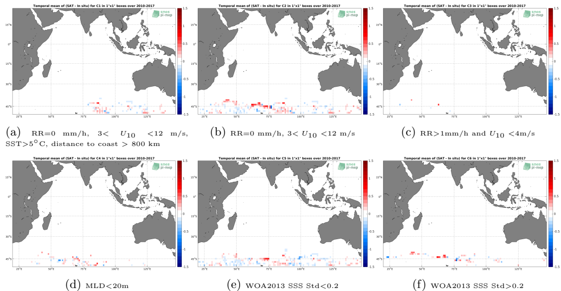
Figure 12: Temporal mean gridded over spatial boxes of size 1^{\circ}\times 1^{\circ} of \Delta\text{SSS} (CCI L4 Merged-OI v1.8 - 7-day running (ESA) - Sea mammals) for 6 different subdatasets corresponding to:RR=0 mm/h, 3 < U_{10} < 12 m/s, SST >5^{\circ}\text{C} , distance to coast > 800 km (a), RR=0 mm/h, 3 < U_{10} < 12 m/s (b), RR >1 mm/h and U_{10} < 4 m/s (c),MLD <20 m (d),WOA2013 SSS Std <0.2 (e),WOA2013 SSS Std >0.2 (f).
