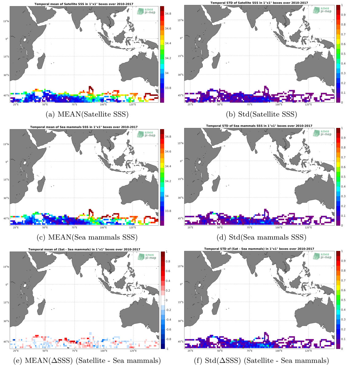
Figure 6: Temporal mean (left) and Std (right) of SSS from CCI L4 Merged-OI v1.8 - 7-day running (ESA) (top), Sea mammals (middle), and of \Delta SSS (Satellite - Sea mammals). Only match-up pairs are used to generate these maps.
