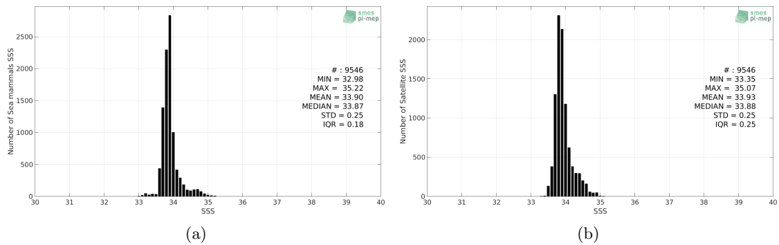
Figure 2: Histograms of SSS from Sea mammals (a) and CCI L4 Merged-OI v1.8 - 7-day running (ESA) (b) considering all match-up pairs per bins of 0.1 over the Indian Ocean Pi-MEP region and for the full satellite product period.
