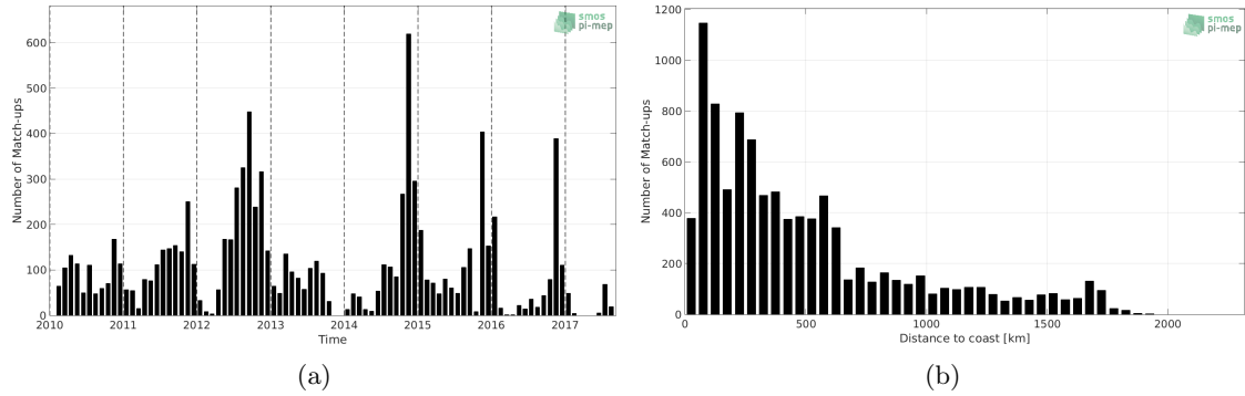
Figure 1: Number of match-ups between Sea mammals and CCI L4 Merged-OI v1.8 - 7-day running (ESA) SSS as a function of time (a) and as function of the distance to coast (b) over the Indian Ocean Pi-MEP region and for the full satellite product period.
