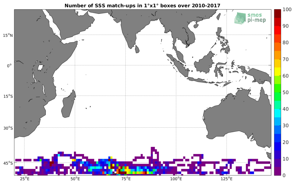
Figure 4: Number of SSS match-ups between Sea mammals SSS and the CCI L4 Merged-OI v1.8 - 7-day running (ESA) SSS product for the Indian Ocean Pi-MEP region over 1°x1° boxes and for the full satellite product period.
