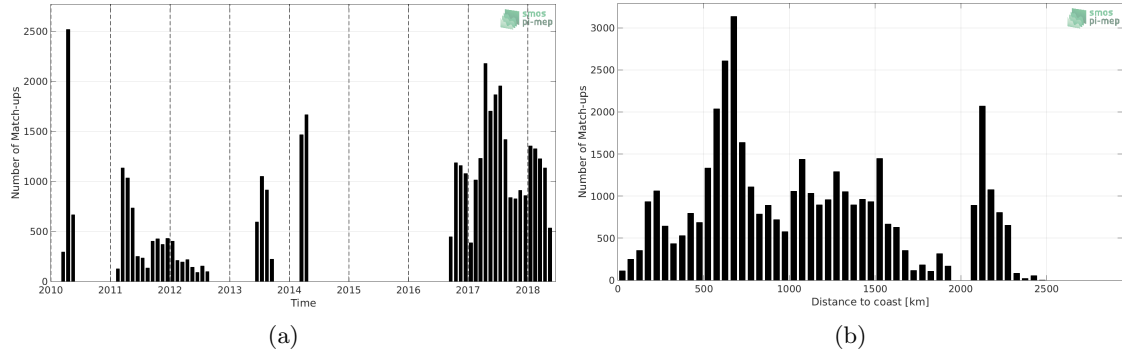
Figure 1: Number of match-ups between Surface drifters and CCI L4 Merged-OI v1.8 - 7-day running (ESA) SSS as a function of time (a) and as function of the distance to coast (b) over the Indian Ocean Pi-MEP region and for the full satellite product period.
