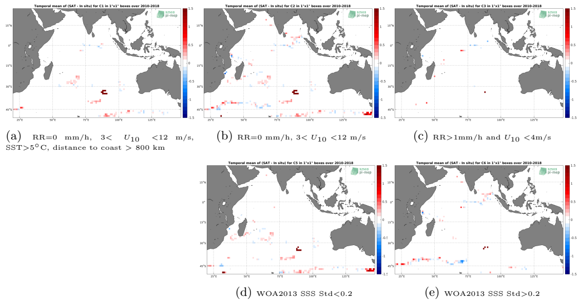
Figure 11: Temporal mean gridded over spatial boxes of size 1^\circ \times 1^\circ of \Delta SSS (CCI L4 Merged-OI v1.8 - 7-day running (ESA) - Surface drifters) for 5 different subdatasets corresponding to: RR=0 mm/h, 3 < U_{10} < 12 m/s, SST > 5^\circ\text{C} , distance to coast > 800 km (a), RR=0 mm/h, 3 < U_{10} < 12 m/s (b), RR > 1 mm/h and U_{10} < 4 m/s (c), WOA2013 SSS Std < 0.2 (d), WOA2013 SSS Std > 0.2 (e).
