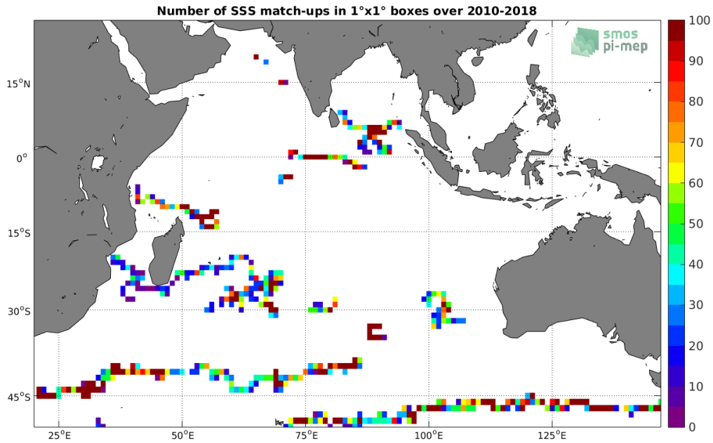
Figure 3: Number of SSS match-ups between Surface drifters SSS and the CCI L4 Merged-OI v1.8 - 7-day running (ESA) SSS product for the Indian Ocean Pi-MEP region over 1^\circ \times 1^\circ boxes and for the full satellite product period.
