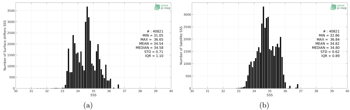
Figure 2: Histograms of SSS from Surface drifters (a) and CCI L4 Merged-OI v1.8 - 7-day running (ESA) (b) considering all match-up pairs per bins of 0.1 over the Indian Ocean Pi-MEP region and for the full satellite product period.
