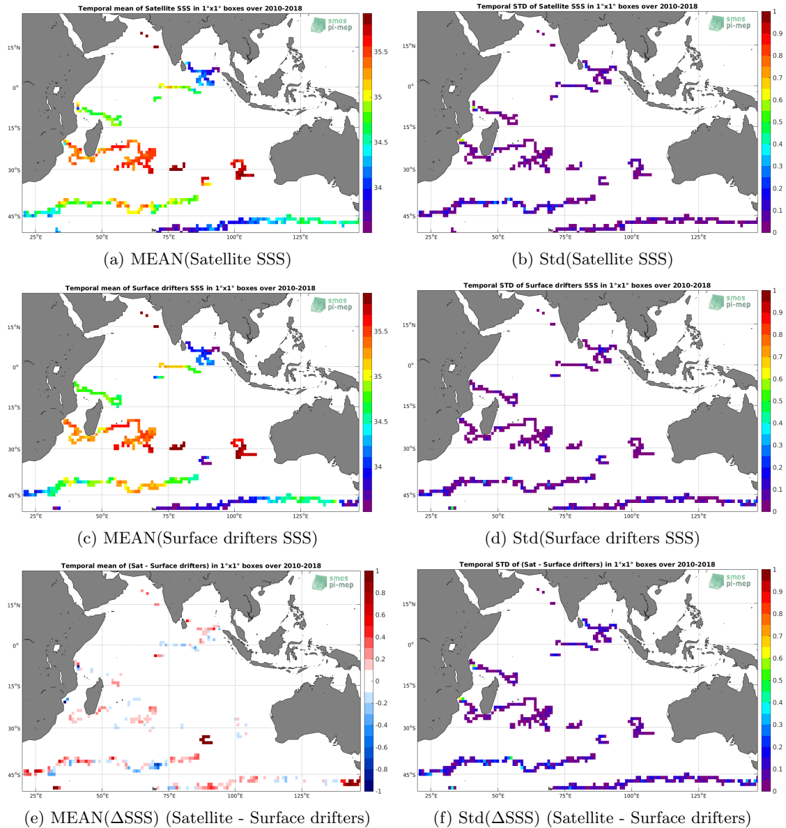
Figure 5: Temporal mean (left) and Std (right) of SSS from CCI L4 Merged-OI v1.8 - 7-day running (ESA) (top), Surface drifters (middle), and of \Delta SSS (Satellite - Surface drifters). Only match-up pairs are used to generate these maps.
