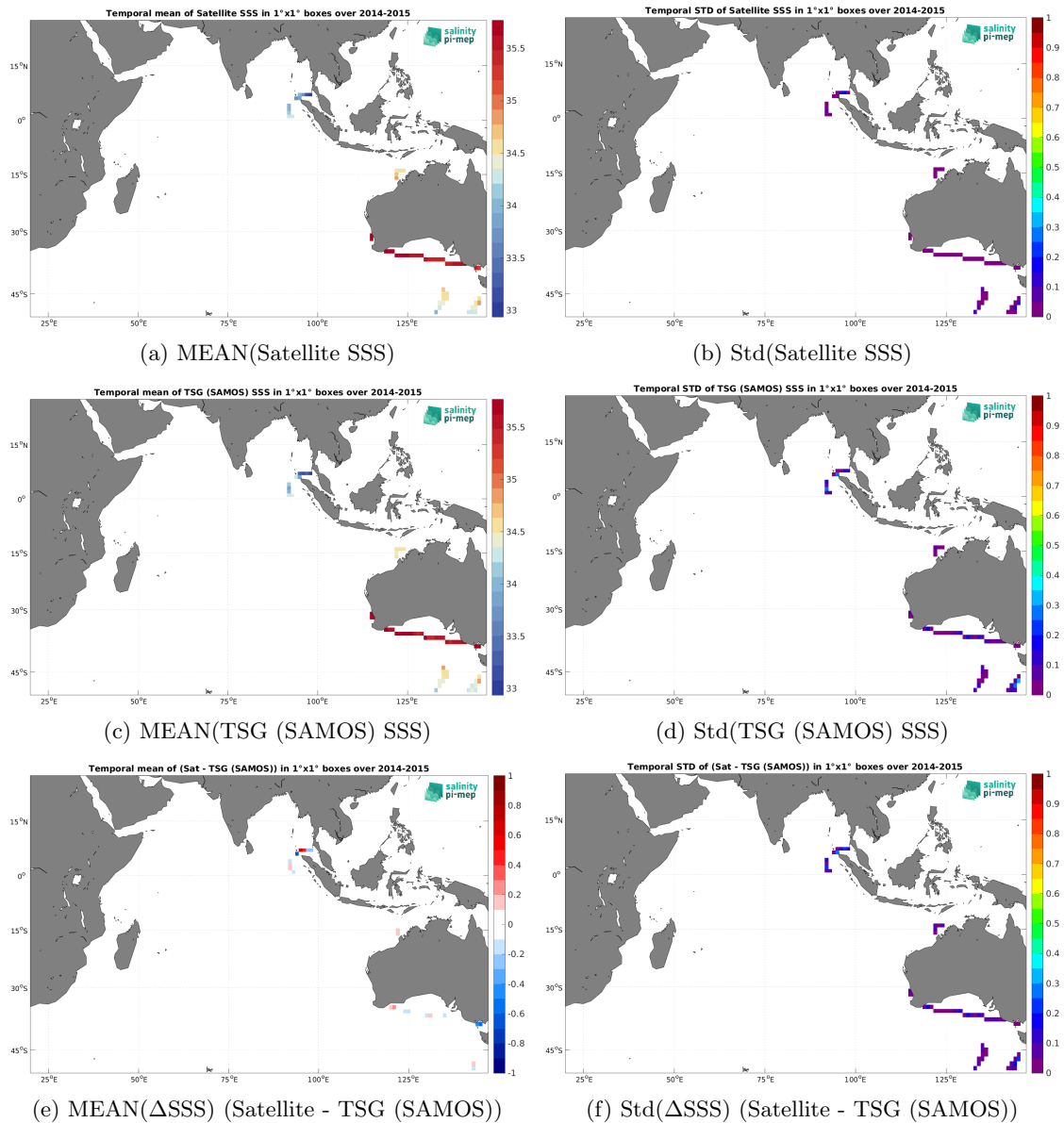
Figure 7: Temporal mean (left) and Std (right) of SSS from Aquarius SSS L4 OI v5 - Weekly (IPRC) (top), TSG (SAMOS) (middle), and of \Delta SSS (Satellite - TSG (SAMOS)). Only match-up pairs are used to generate these maps.
