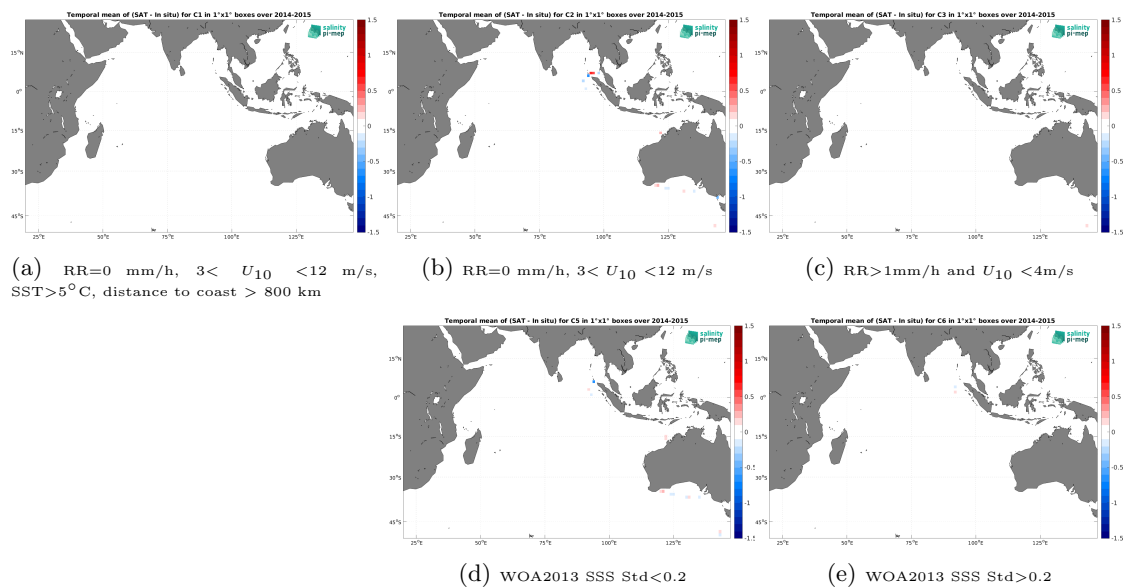
Figure 14: Temporal mean gridded over spatial boxes of size 1^\circ \times 1^\circ of \Delta SSS (Aquarius SSS L4 OI v5 - Weekly (IPRC) - TSG (SAMOS)) for 5 different subdatasets corresponding to:RR=0 mm/h, 3 < U_{10} < 12 m/s, SST >5^\circ C, distance to coast > 800 km (a), RR=0 mm/h, 3 < U_{10} < 12 m/s (b), RR >1 mm/h and U_{10} < 4 m/s (c), WOA2013 SSS Std <0.2 (d), WOA2013 SSS Std >0.2 (e).
