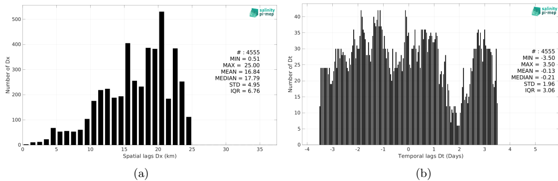
Figure 6: Histograms of the spatial (a) and temporal (b) lags between the location/time of the TSG (SAMOS) measurement and the date of the corresponding Aquarius SSS L4 OI v5 - Weekly (IPRC) SSS pixel.
