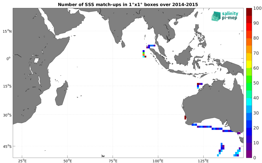
Figure 5: Number of SSS match-ups between TSG (SAMOS) SSS and the Aquarius SSS L4 OI v5 - Weekly (IPRC) SSS product for the Indian Ocean Pi-MEP region over 1^\circ \times 1^\circ boxes and for the full satellite product period.
