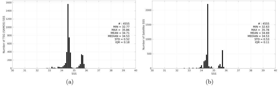
Figure 3: Histograms of SSS from TSG (SAMOS) (a) and Aquarius SSS L4 OI v5 - Weekly (IPRC) (b) considering all match-up pairs per bins of 0.1 over the Indian Ocean Pi-MEP region and for the full satellite product period.
