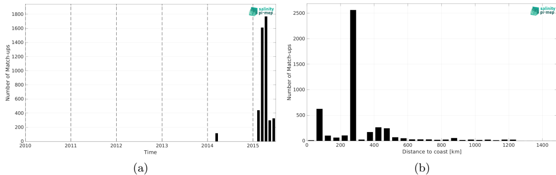
Figure 2: Number of match-ups between TSG (SAMOS) and Aquarius SSS L4 OI v5 - Weekly (IPRC) SSS as a function of time (a) and as function of the distance to coast (b) over the Indian Ocean Pi-MEP region and for the full satellite product period.
