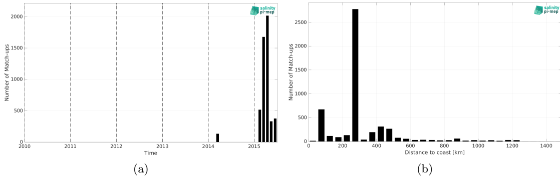
Figure 1: Number of match-ups between TSG (SAMOS) and Aquarius SSS L4 OI v5 - Weekly (IPRC) SSS as a function of time (a) and as function of the distance to coast (b) over the Indian Ocean Pi-MEP region and for the full satellite product period.
