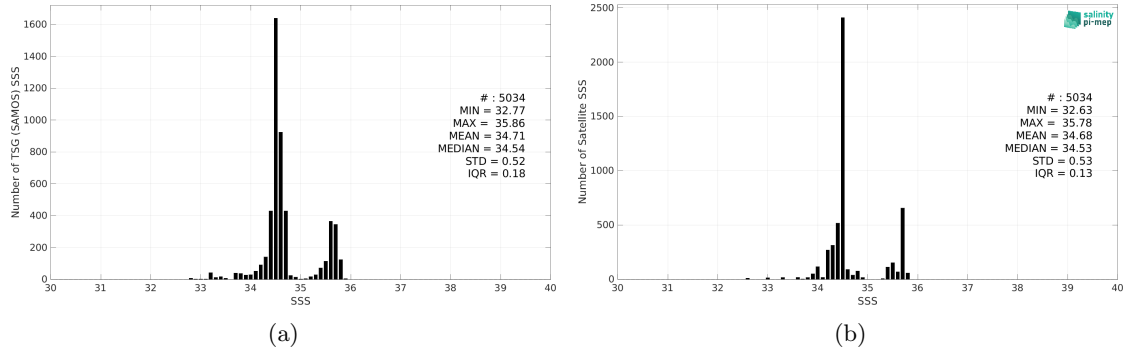
Figure 2: Histograms of SSS from TSG (SAMOS) (a) and Aquarius SSS L4 OI v5 - Weekly (IPRC) (b) considering all match-up pairs per bins of 0.1 over the Indian Ocean Pi-MEP region and for the full satellite product period.
