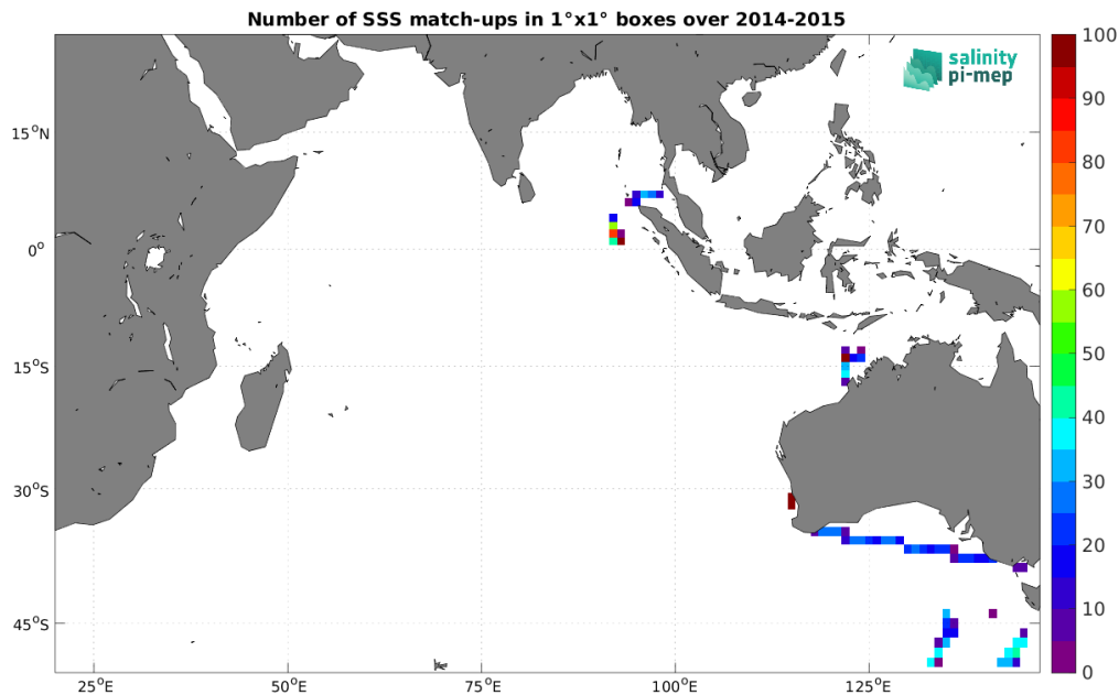
Figure 4: Number of SSS match-ups between TSG (SAMOS) SSS and the Aquarius SSS L4 OI v5 - Weekly (IPRC) SSS product for the Indian Ocean Pi-MEP region over 1^\circ \times 1^\circ boxes and for the full satellite product period.
