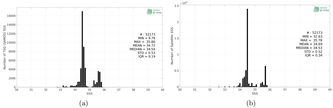
Figure 2: Histograms of SSS from TSG (SAMOS) (a) and Aquarius SSS L4 OI v5 - Weekly (IPRC) (b) considering all match-up pairs per bins of 0.1 over the Indian Ocean Pi-MEP region and for the full satellite product period.
