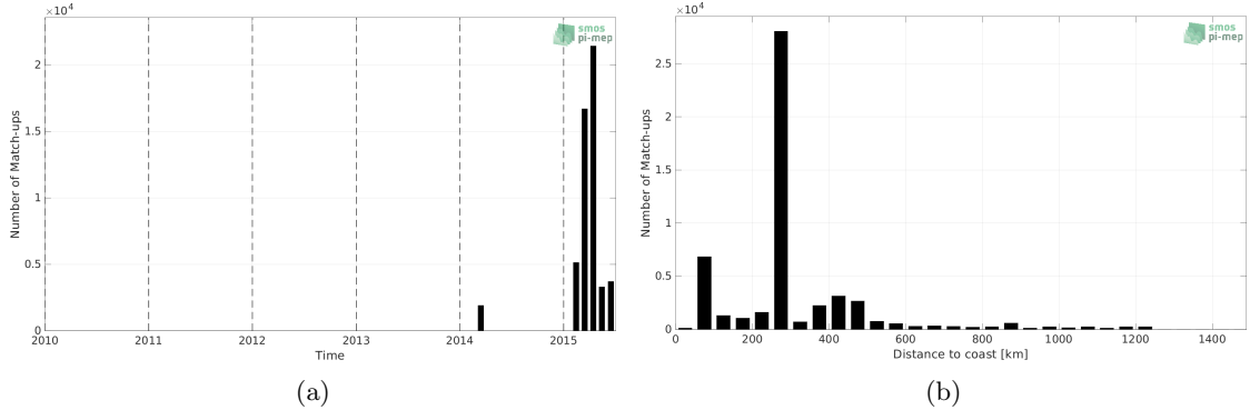
Figure 1: Number of match-ups between TSG (SAMOS) and Aquarius SSS L4 OI v5 - Weekly (IPRC) SSS as a function of time (a) and as function of the distance to coast (b) over the Indian Ocean Pi-MEP region and for the full satellite product period.
