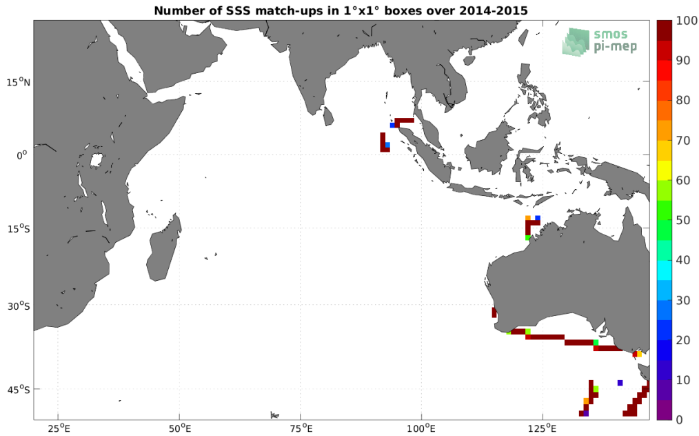
Figure 4: Number of SSS match-ups between TSG (SAMOS) SSS and the Aquarius SSS L4 OI v5 - Weekly (IPRC) SSS product for the Indian Ocean Pi-MEP region over 1^\circ \times 1^\circ boxes and for the full satellite product period.
