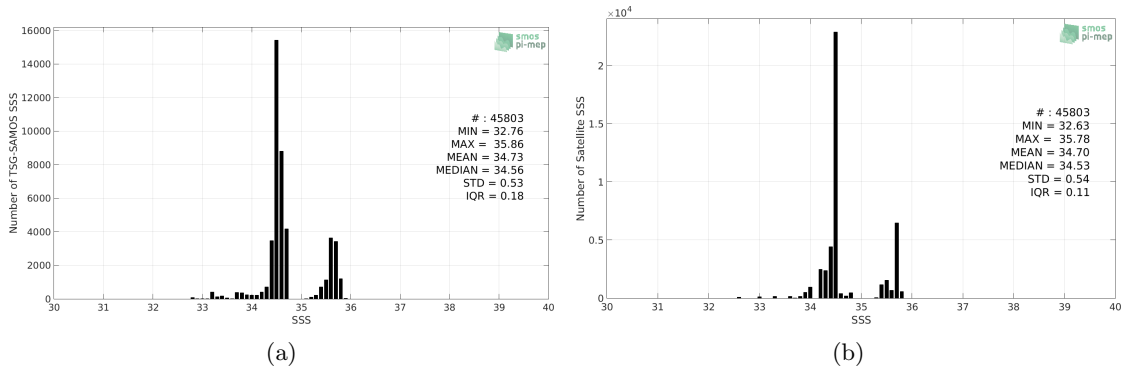
Figure 2: Histograms of SSS from TSG-SAMOS (a) and Aquarius-L4-IPRC-V5-WEEKLY (b) considering all match-up pairs per bins of 0.1 over the Indian Ocean Pi-MEP region and for the full satellite product period.
