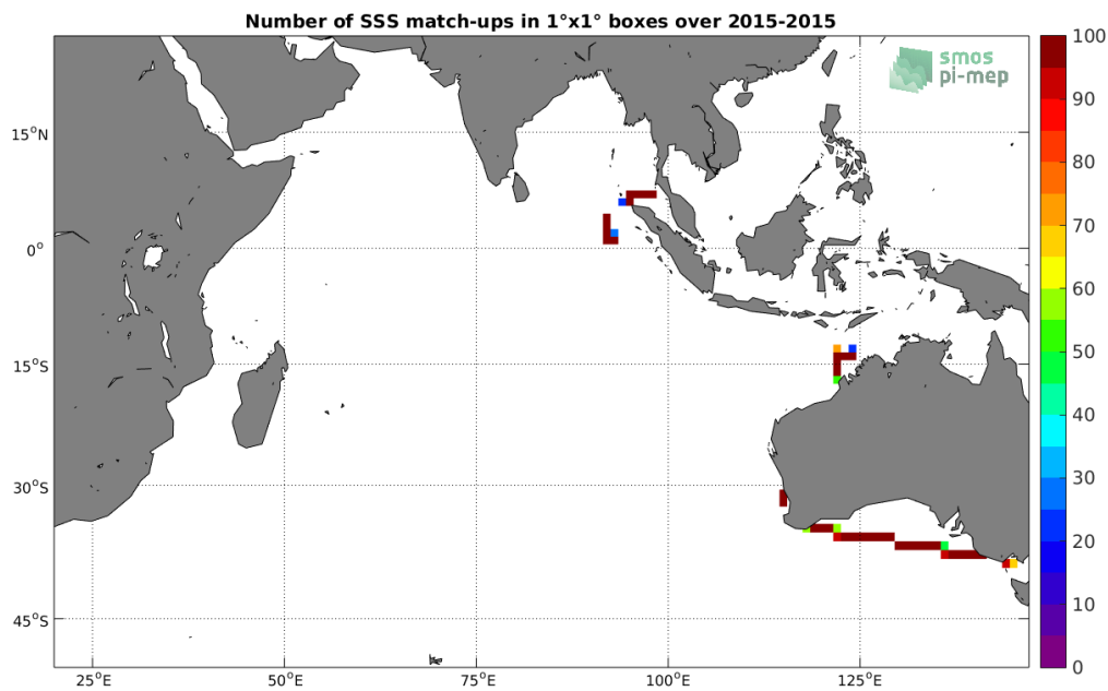
Figure 4: Number of SSS match-ups between TSG-SAMOS SSS and the Aquarius-L4-IPRC-V5-WEEKLY SSS product for the Indian Ocean Pi-MEP region over 1^\circ \times 1^\circ boxes and for the full satellite product period.
