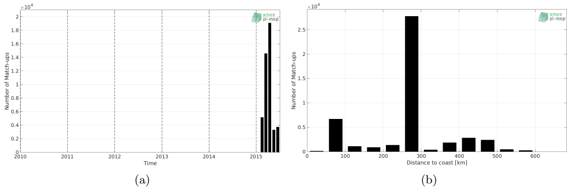
Figure 1: Number of match-ups between TSG-SAMOS and Aquarius-L4-IPRC-V5-WEEKLY SSS as a function of time (a) and as function of the distance to coast (b) over the Indian Ocean Pi-MEP region and for the full satellite product period.
