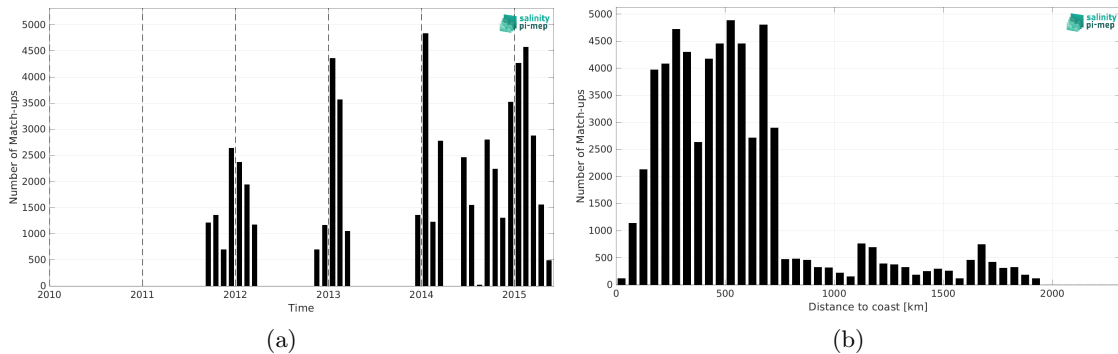
Figure 2: Number of match-ups between TSG (LEGOS-DM) and Aquarius SSS L4 OI v5 - Weekly (IPRC) SSS as a function of time (a) and as function of the distance to coast (b) over the Indian Ocean Pi-MEP region and for the full satellite product period.
