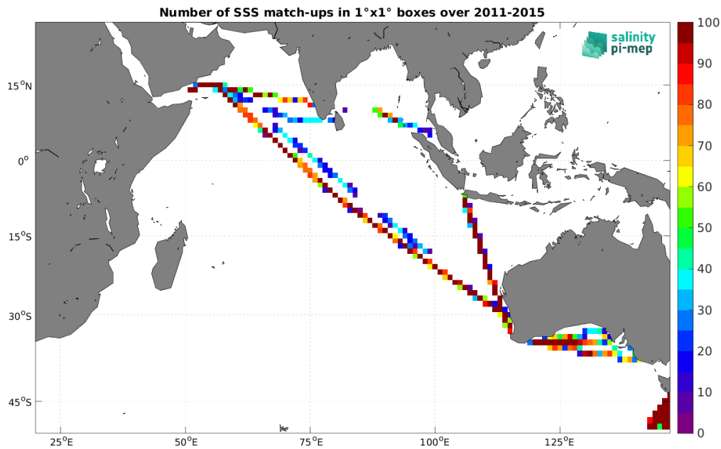
Figure 5: Number of SSS match-ups between TSG (LEGOS-DM) SSS and the Aquarius SSS L4 OI v5 - Weekly (IPRC) SSS product for the Indian Ocean Pi-MEP region over 1^\circ \times 1^\circ boxes and for the full satellite product period.
