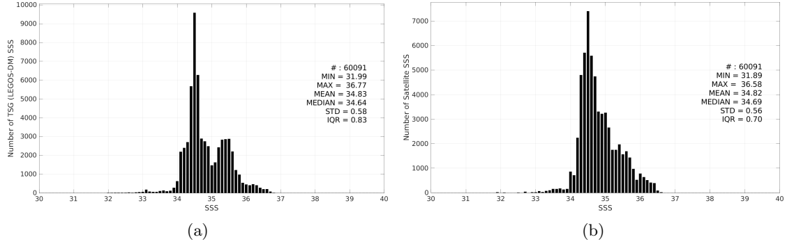
Figure 3: Histograms of SSS from TSG (LEGOS-DM) (a) and Aquarius SSS L4 OI v5 - Weekly (IPRC) (b) considering all match-up pairs per bins of 0.1 over the Indian Ocean Pi-MEP region and for the full satellite product period.
