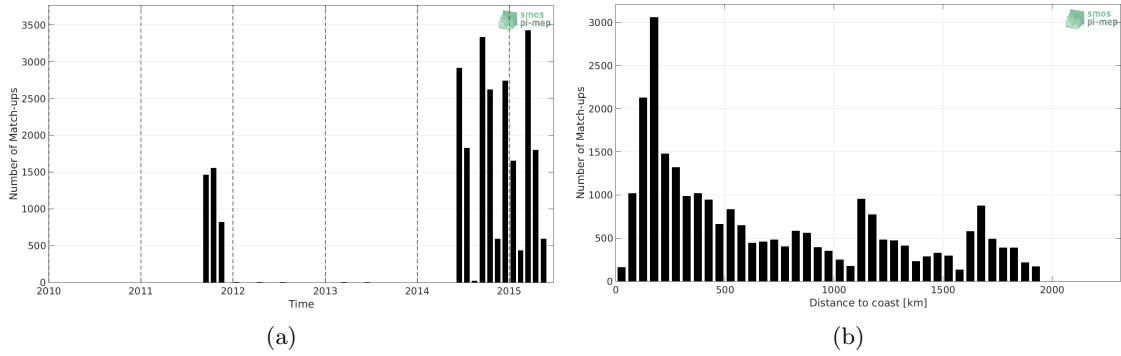
Figure 1: Number of match-ups between TSG-LEGOS-DM and Aquarius-L4-IPRC-V5-WEEKLY SSS as a function of time (a) and as function of the distance to coast (b) over the Indian Ocean Pi-MEP region and for the full satellite product period.
