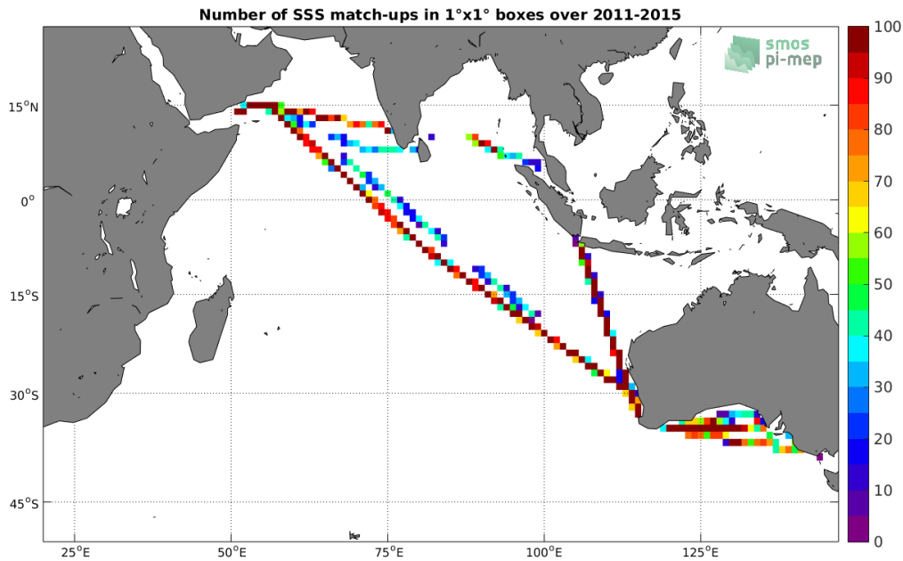
Figure 4: Number of SSS match-ups between TSG-LEGOS-DM SSS and the Aquarius-L4-IPRC-V5-WEEKLY SSS product for the Indian Ocean Pi-MEP region over 1°x1° boxes and for the full satellite product period.
