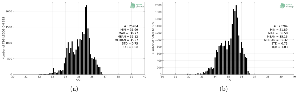
Figure 2: Histograms of SSS from TSG-LEGOS-DM (a) and Aquarius-L4-IPRC-V5-WEEKLY (b) considering all match-up pairs per bins of 0.1 over the Indian Ocean Pi-MEP region and for the full satellite product period.
