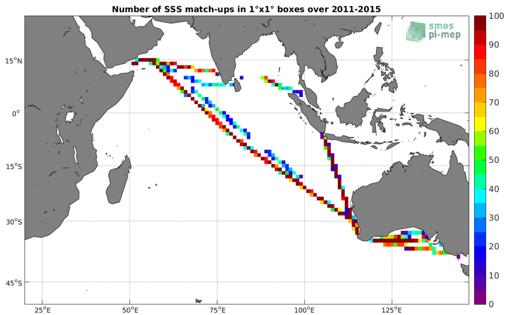
Figure 4: Number of SSS match-ups between TSG-LEGOS-DM SSS and the Aquarius-L4-IPRC-V5-WEEKLY SSS product for the Indian Ocean Pi-MEP region over 1^\circ \times 1^\circ boxes and for the full satellite product period.
