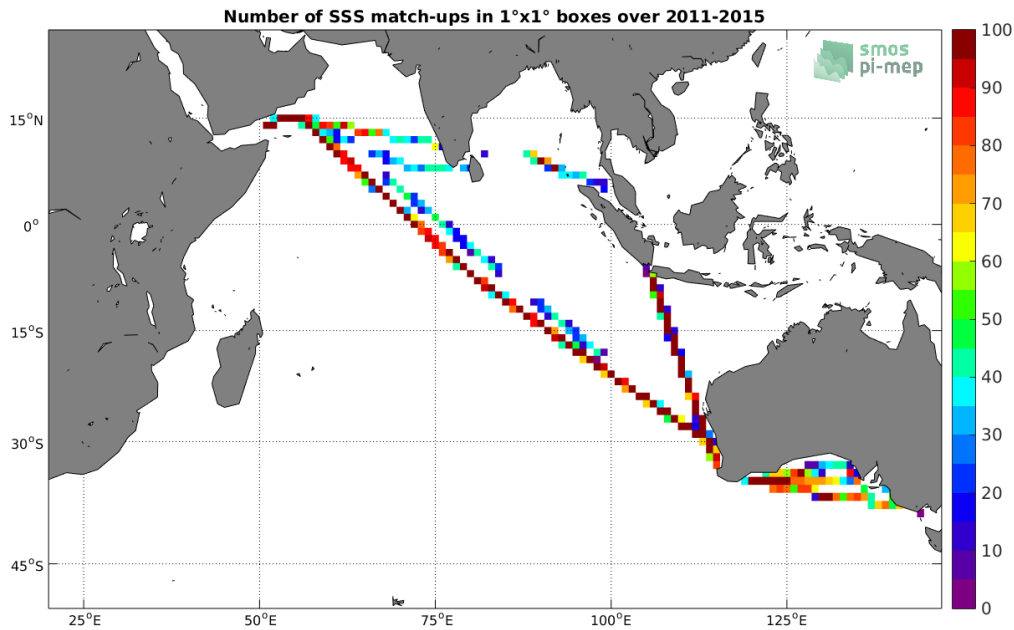
Figure 4: Number of SSS match-ups between TSG-LEGOS-DM SSS and the Aquarius-L4-IPRC-V5-WEEKLY SSS product for the Indian Ocean Pi-MEP region over 1^\circ \times 1^\circ boxes and for the full satellite product period.
