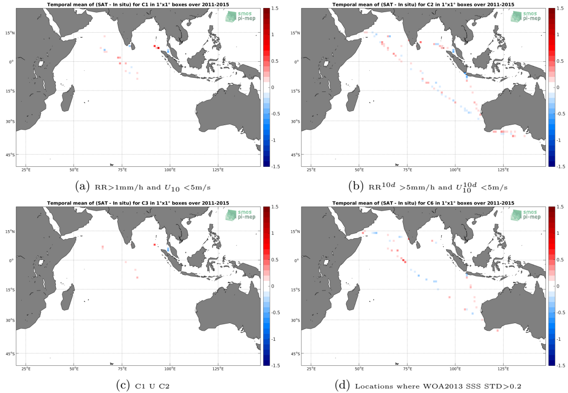
Figure 12: Temporal mean gridded over spatial boxes of size 1^\circ \times 1^\circ of \Delta SSS (Aquarius-L4-IPRC-V5-WEEKLY - TSG-LEGOS-DM) for 4 different subdatasets corresponding to: RR > 1mm/h and U_{10} < 5\text{m/s} (a), RR^{10d} > 5\text{mm/h} and U_{10}^{10d} < 5\text{m/s} (b), C1 U C2 (c), Locations where WOA2013 SSS STD > 0.2 (d).
