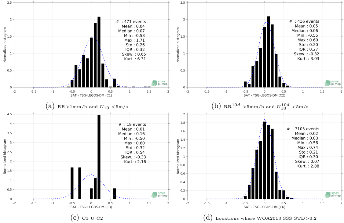
Figure 13: Normalized histogram of \Delta SSS (Aquarius-L4-IPRC-V5-WEEKLY - TSG-LEGOS-DM) for 6 different subdatasets corresponding to: RR > 1mm/h and U_{10} < 5 m/s (a), RR^{10d} > 5 mm/h and U_{10}^{10d} < 5 m/s (b), C1 U C2 (c), Locations where WOA2013 SSS STD > 0.2 (d).
