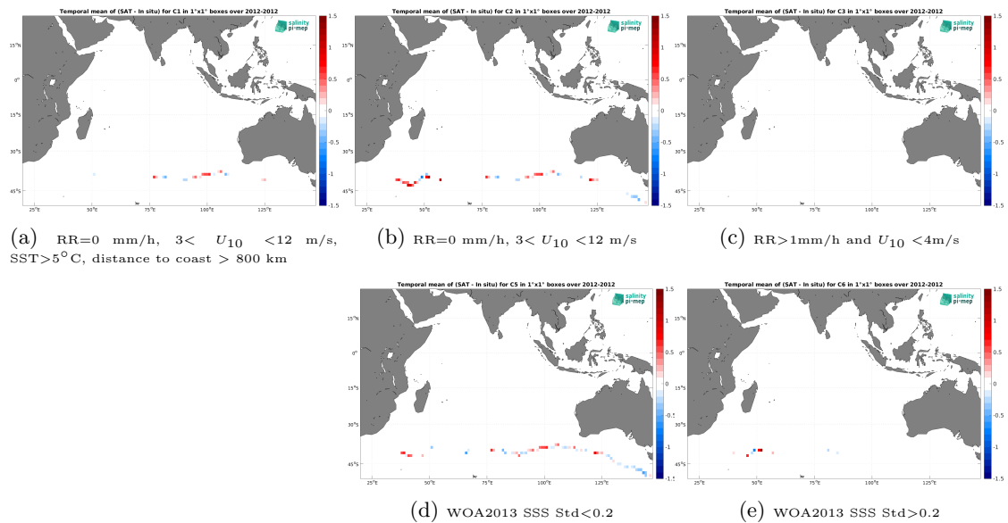
Figure 14: Temporal mean gridded over spatial boxes of size 1^\circ \times 1^\circ of \Delta SSS (Aquarius SSS L4 OI v5 - Weekly (IPRC) - TSG (GOSUD-Sailing-ship)) for 5 different subdatasets corresponding to: RR=0 mm/h, 3 < U_{10} < 12 m/s, SST > 5^\circ\text{C} , distance to coast > 800 km (a), RR=0 mm/h, 3 < U_{10} < 12 m/s (b), RR > 1\text{mm/h} and U_{10} < 4\text{m/s} (c), WOA2013 SSS Std < 0.2 (d), WOA2013 SSS Std > 0.2 (e).
