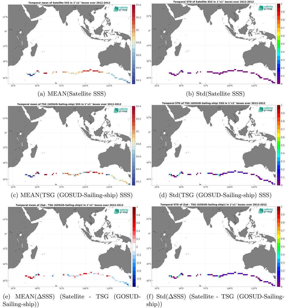
Figure 7: Temporal mean (left) and Std (right) of SSS from Aquarius SSS L4 OI v5 - Weekly (IPRC) (top), TSG (GOSUD-Sailing-ship) (middle), and of \Delta SSS (Satellite - TSG (GOSUD-Sailing-ship)). Only match-up pairs are used to generate these maps.
