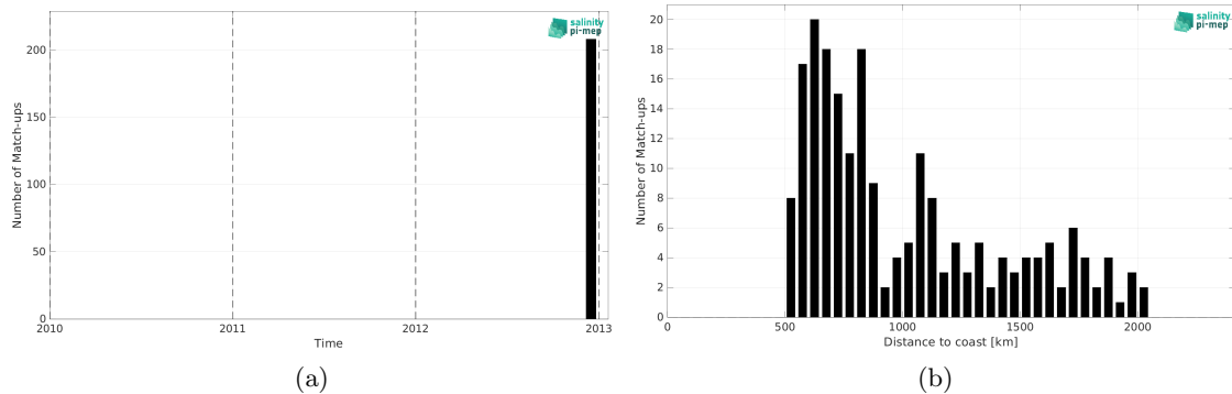
Figure 2: Number of match-ups between TSG (GOSUD-Sailing-ship) and Aquarius SSS L4 OI v5 - Weekly (IPRC) SSS as a function of time (a) and as function of the distance to coast (b) over the Indian Ocean Pi-MEP region and for the full satellite product period.
