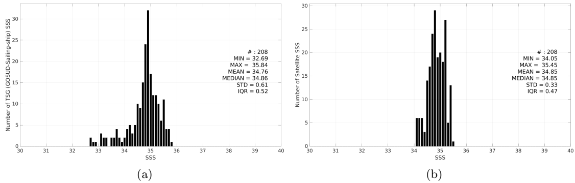
Figure 3: Histograms of SSS from TSG (GOSUD-Sailing-ship) (a) and Aquarius SSS L4 OI v5 - Weekly (IPRC) (b) considering all match-up pairs per bins of 0.1 over the Indian Ocean Pi-MEP region and for the full satellite product period.
