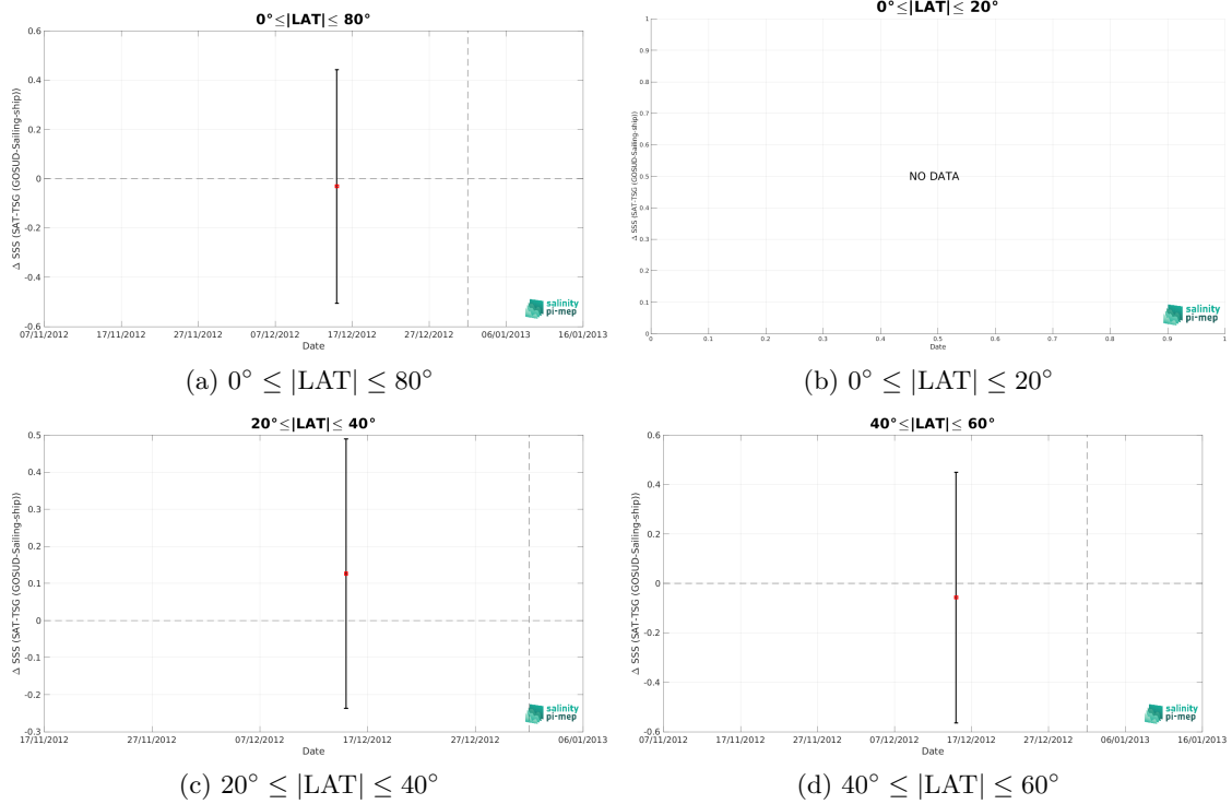
Figure 11: Monthly median (red curves) of \Delta\text{SSS} (Satellite - TSG (GOSUD-Sailing-ship)) and \pm 1 Std (black vertical thick bars) as function of time for all the collected Pi-MEP match-up pairs estimated over the Indian Ocean Pi-MEP region and for the full satellite product period are shown for different latitude bands: (a) 80°S-80°N, (b) 20°S-20°N, (c) 40°S-20°S and 20°N-40°N and (d) 60°S-40°S and 40°N-60°N.
