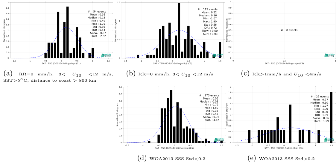
Figure 15: Normalized histogram of \Delta SSS (Aquarius SSS L4 OI v5 - Weekly (IPRC) - TSG (GOSUD-Sailing-ship)) for 5 different subdatasets corresponding to: RR=0 mm/h, 3 < U_{10} < 12 m/s, SST>5°C, distance to coast > 800 km (a), RR=0 mm/h, 3 < U_{10} < 12 m/s (b), RR>1mm/h and U_{10} < 4 m/s (c), WOA2013 SSS Std<0.2 (d), WOA2013 SSS Std>0.2 (e).
