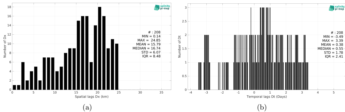
Figure 6: Histograms of the spatial (a) and temporal (b) lags between the location/time of the TSG (GOSUD-Sailing-ship) measurement and the date of the corresponding Aquarius SSS L4 OI v5 - Weekly (IPRC) SSS pixel.
