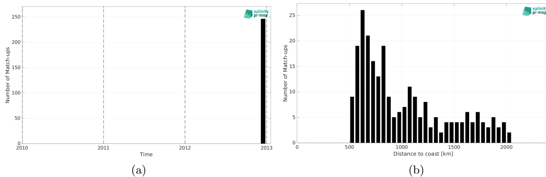
Figure 1: Number of match-ups between TSG (GOSUD-Sailing-ship) and Aquarius SSS L4 OI v5 - Weekly (IPRC) SSS as a function of time (a) and as function of the distance to coast (b) over the Indian Ocean Pi-MEP region and for the full satellite product period.
