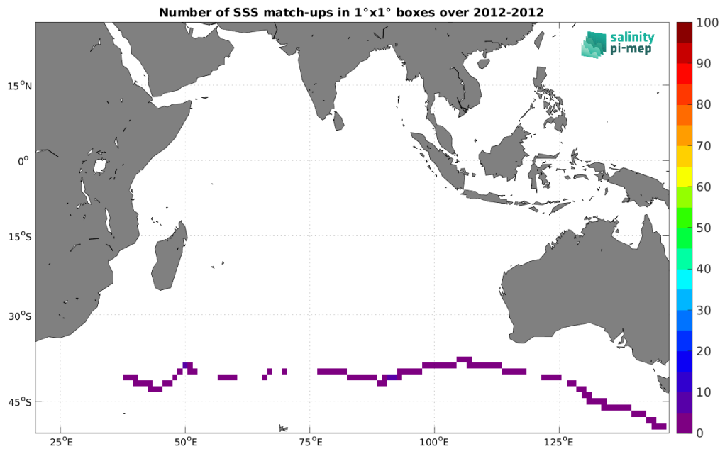
Figure 4: Number of SSS match-ups between TSG (GOSUD-Sailing-ship) SSS and the Aquarius SSS L4 OI v5 - Weekly (IPRC) SSS product for the Indian Ocean Pi-MEP region over 1^\circ \times 1^\circ boxes and for the full satellite product period.
