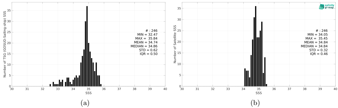
Figure 2: Histograms of SSS from TSG (GOSUD-Sailing-ship) (a) and Aquarius SSS L4 OI v5 - Weekly (IPRC) (b) considering all match-up pairs per bins of 0.1 over the Indian Ocean Pi-MEP region and for the full satellite product period.
