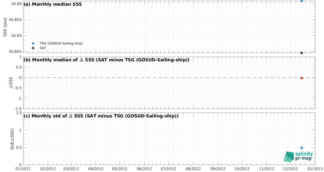
Figure 7: Time series of the monthly median SSS (top), median of \Delta SSS (Satellite - TSG (GOSUD-Sailing-ship)) and Std of \Delta SSS (Satellite - TSG (GOSUD-Sailing-ship)) over the Indian Ocean Pi-MEP region considering all match-ups collected by the Pi-MEP.
