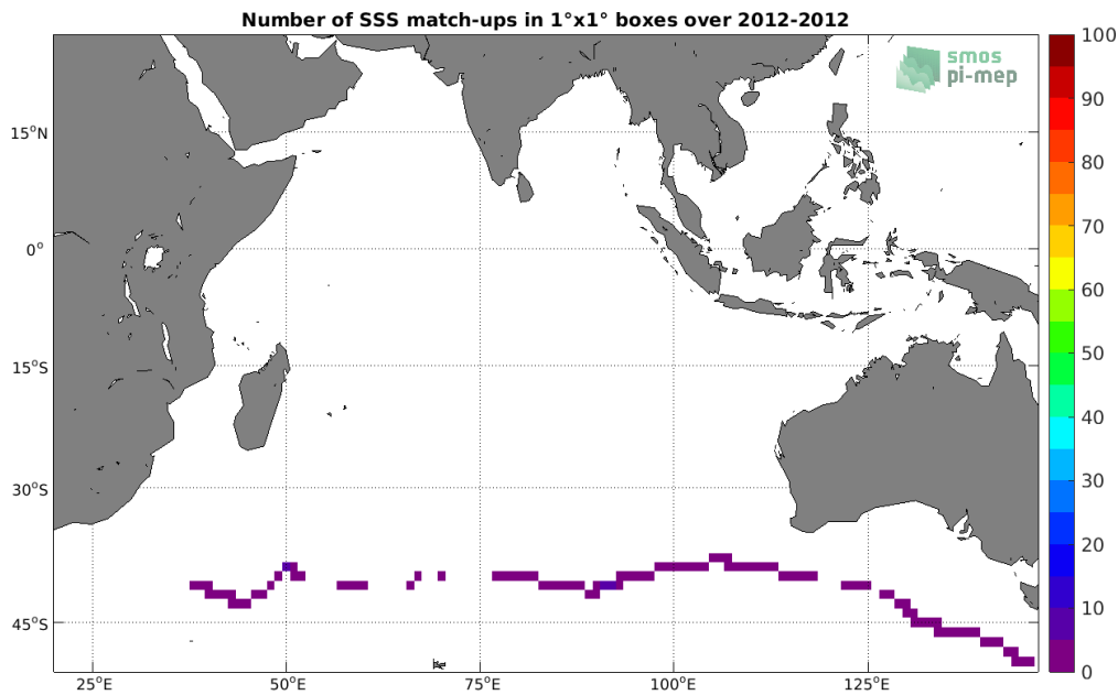
Figure 4: Number of SSS match-ups between TSG (GOSUD-Sailing-ship) SSS and the Aquarius SSS L4 OI v5 - Weekly (IPRC) SSS product for the Indian Ocean Pi-MEP region over 1°x1° boxes and for the full satellite product period.
