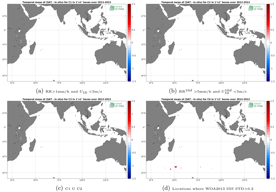
Figure 12: Temporal mean gridded over spatial boxes of size 1^\circ \times 1^\circ of \Delta SSS (Aquarius-L4-IPRC-V5-WEEKLY - TSG-GOSUD-Sailing-ship) for 4 different subdatasets corresponding to: RR > 1\text{mm/h} and U_{10} < 5\text{m/s} (a), RR^{10d} > 5\text{mm/h} and U_{10}^{10d} < 5\text{m/s} (b), C1 U C2 (c), Locations where WOA2013 SSS STD > 0.2 (d).
