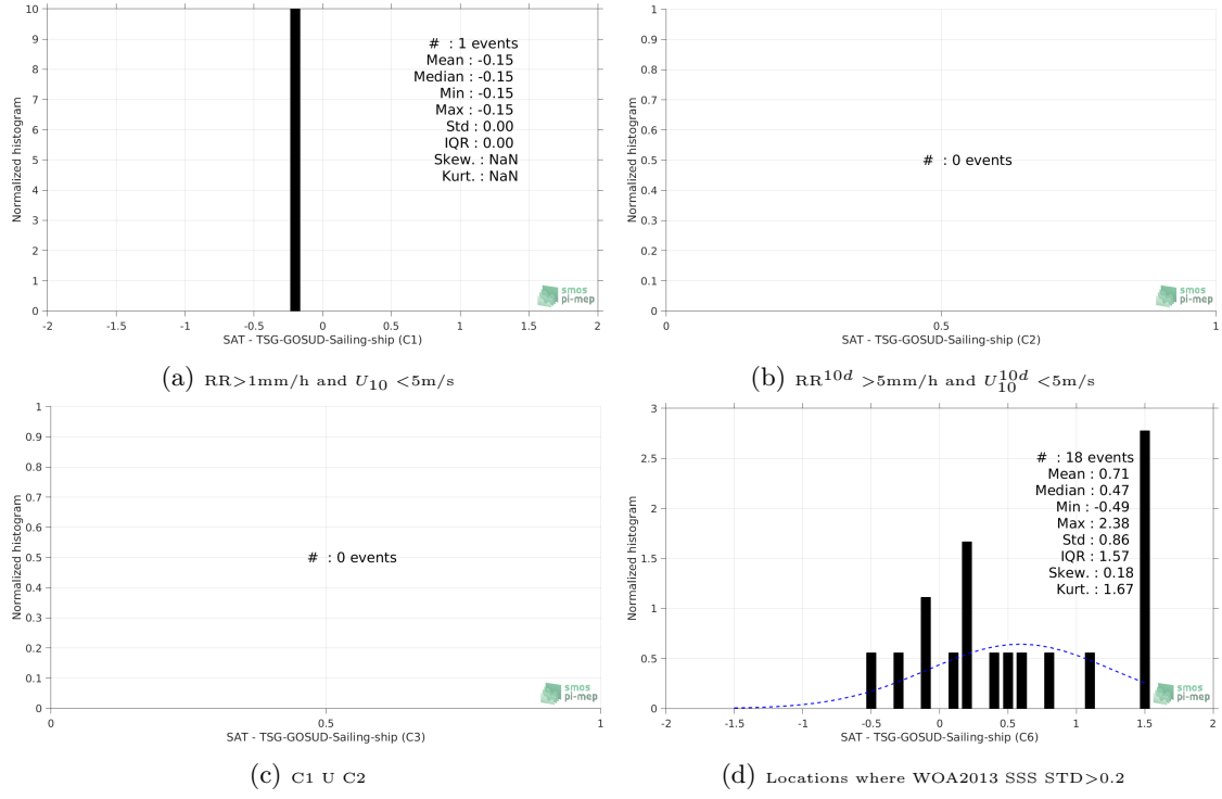
Figure 13: Normalized histogram of \Delta\text{SSS} (Aquarius-L4-IPRC-V5-WEEKLY - TSG-GOSUD-Sailing-ship) for 6 different subdatasets corresponding to: RR > 1\text{mm/h} and U_{10} < 5\text{m/s} (a), RR^{10d} > 5\text{mm/h} and U_{10}^{10d} < 5\text{m/s} (b), C1 \cup C2 (c), Locations where WOA2013 SSS STD > 0.2 (d).
