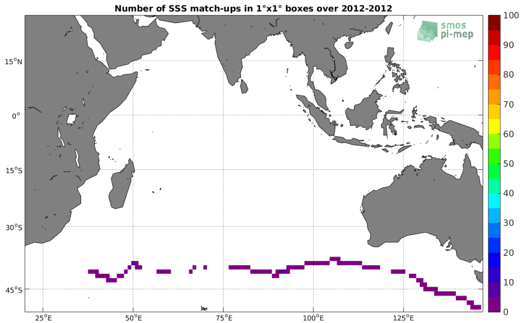
Figure 4: Number of SSS match-ups between TSG-GOSUD-Sailing-ship SSS and the Aquarius-L4-IPRC-V5-WEEKLY SSS product for the Indian Ocean Pi-MEP region over 1°x1° boxes and for the full satellite product period.
