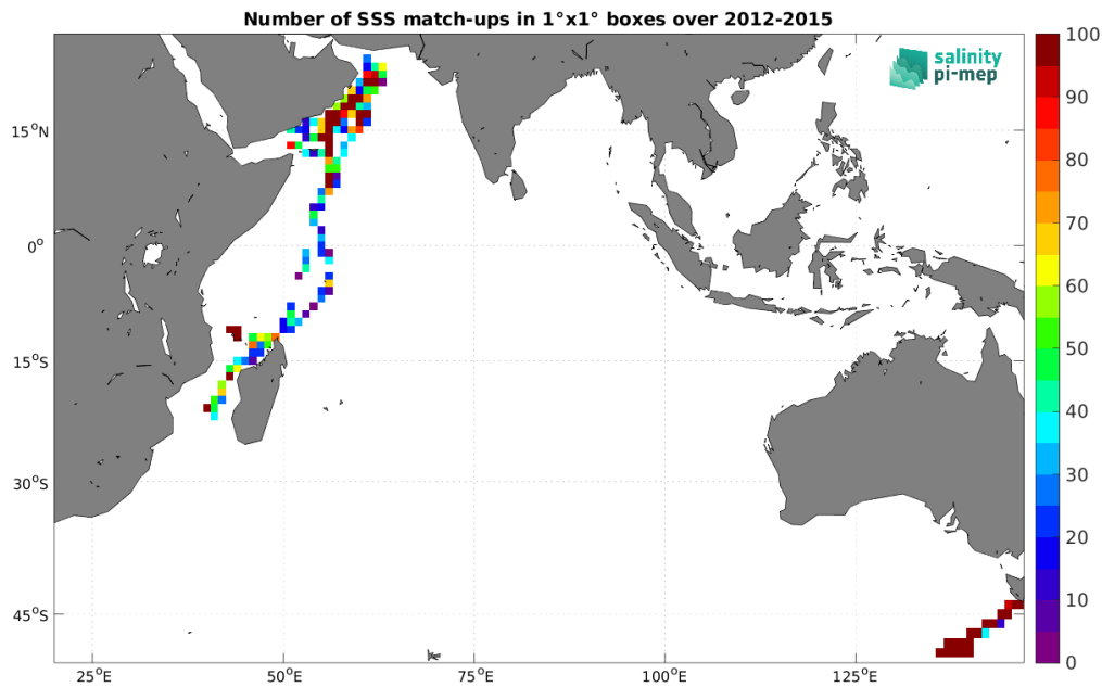
Figure 5: Number of SSS match-ups between TSG (GOSUD-Research-vessel) SSS and the Aquarius SSS L4 OI v5 - Weekly (IPRC) SSS product for the Indian Ocean Pi-MEP region over 1^\circ \times 1^\circ boxes and for the full satellite product period.
