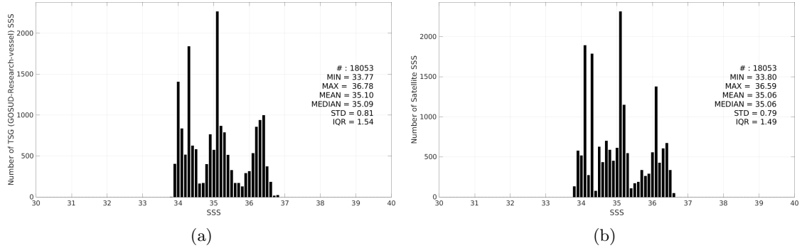
Figure 3: Histograms of SSS from TSG (GOSUD-Research-vessel) (a) and Aquarius SSS L4 OI v5 - Weekly (IPRC) (b) considering all match-up pairs per bins of 0.1 over the Indian Ocean Pi-MEP region and for the full satellite product period.
