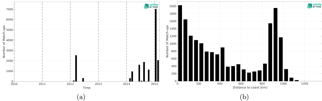
Figure 2: Number of match-ups between TSG (GOSUD-Research-vessel) and Aquarius SSS L4 OI v5 - Weekly (IPRC) SSS as a function of time (a) and as function of the distance to coast (b) over the Indian Ocean Pi-MEP region and for the full satellite product period.
