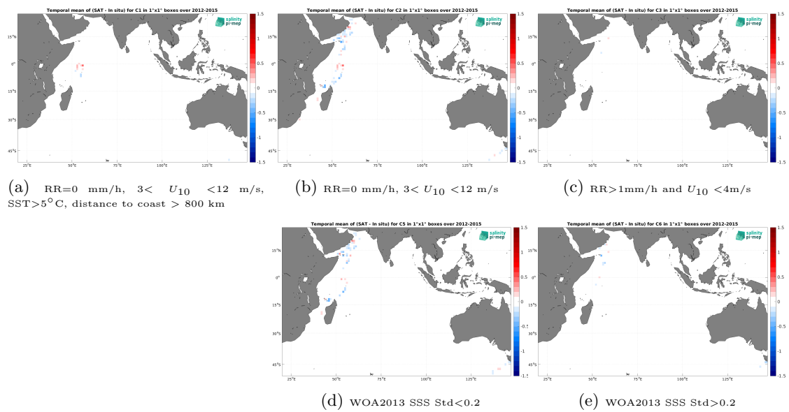
Figure 12: Temporal mean gridded over spatial boxes of size 1^\circ \times 1^\circ of \Delta\text{SSS} (Aquarius SSS L4 OI v5 - Weekly (IPRC) - TSG (GOSUD-Research-vessel)) for 5 different subdatasets corresponding to:RR=0 mm/h, 3 < U_{10} < 12 m/s, SST >5^\circ\text{C} , distance to coast > 800 km (a), RR=0 mm/h, 3 < U_{10} < 12 m/s (b), RR >1 mm/h and U_{10} < 4 m/s (c), WOA2013 SSS Std <0.2 (d), WOA2013 SSS Std >0.2 (e).
