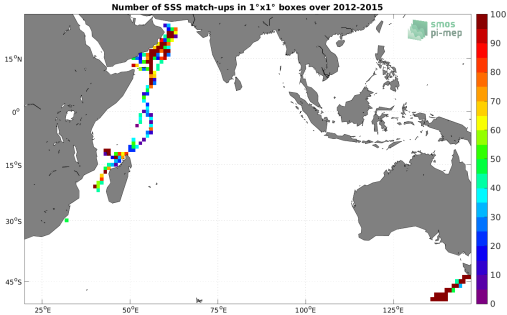
Figure 4: Number of SSS match-ups between TSG (GOSUD-Research-vessel) SSS and the Aquarius SSS L4 OI v5 - Weekly (IPRC) SSS product for the Indian Ocean Pi-MEP region over 1^\circ \times 1^\circ boxes and for the full satellite product period.
