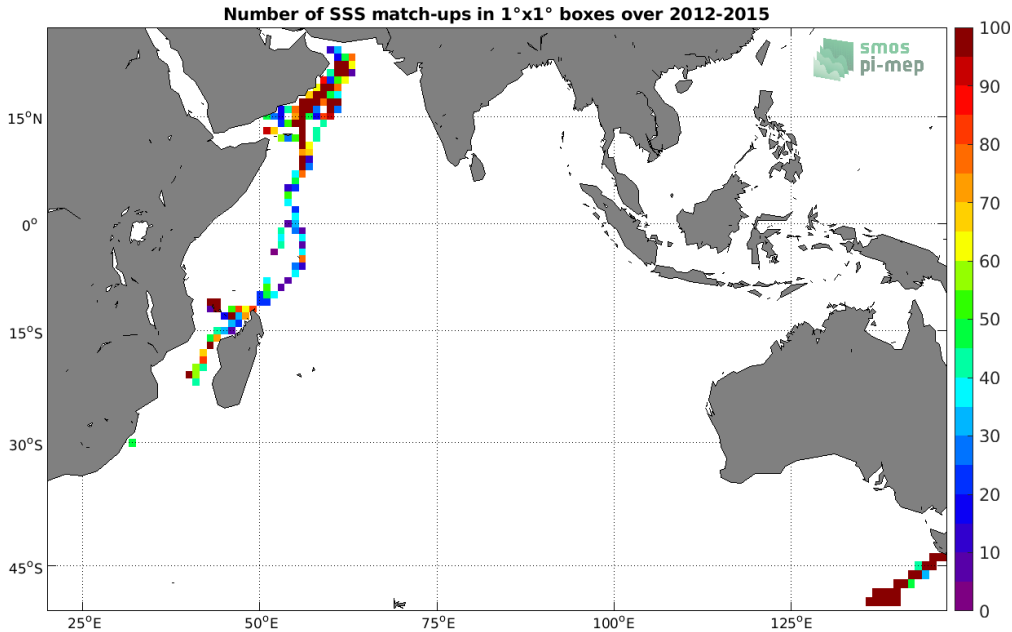
Figure 4: Number of SSS match-ups between TSG (GOSUD-Research-vessel) SSS and the Aquarius SSS L4 OI v5 - Weekly (IPRC) SSS product for the Indian Ocean Pi-MEP region over 1^{\circ} \times 1^{\circ} boxes and for the full satellite product period.
