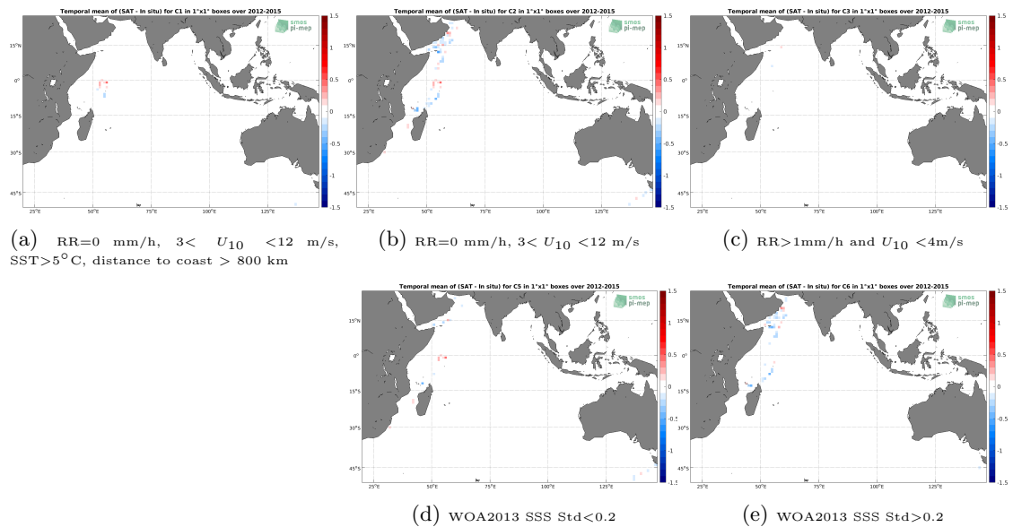
Figure 12: Temporal mean gridded over spatial boxes of size 1°x1° of \Delta SSS (Aquarius SSS L4 OI v5 - Weekly (IPRC) - TSG (GOSUD-Research-vessel)) for 5 different subdatasets corresponding to:RR=0 mm/h, 3 < U_{10} < 12 m/s, SST>5°C, distance to coast > 800 km (a), RR=0 mm/h, 3 < U_{10} < 12 m/s (b), RR>1mm/h and U_{10} < 4 m/s (c), WOA2013 SSS Std<0.2 (d), WOA2013 SSS Std>0.2 (e).
