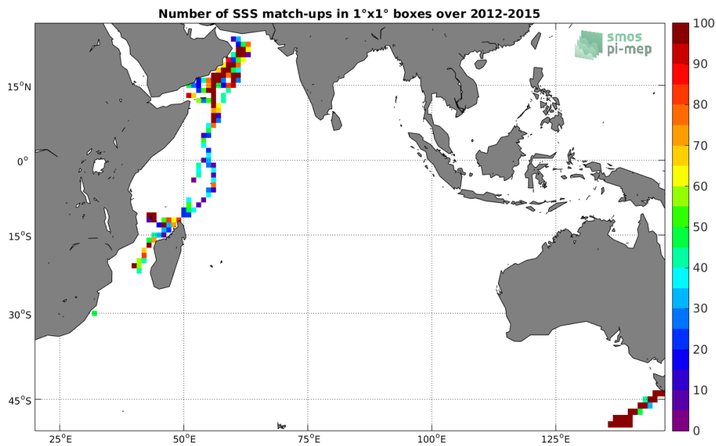
Figure 4: Number of SSS match-ups between TSG-GOSUD-Research-vessel SSS and the Aquarius-L4-IPRC-V5-WEEKLY SSS product for the Indian Ocean Pi-MEP region over 1^\circ \times 1^\circ boxes and for the full satellite product period.
