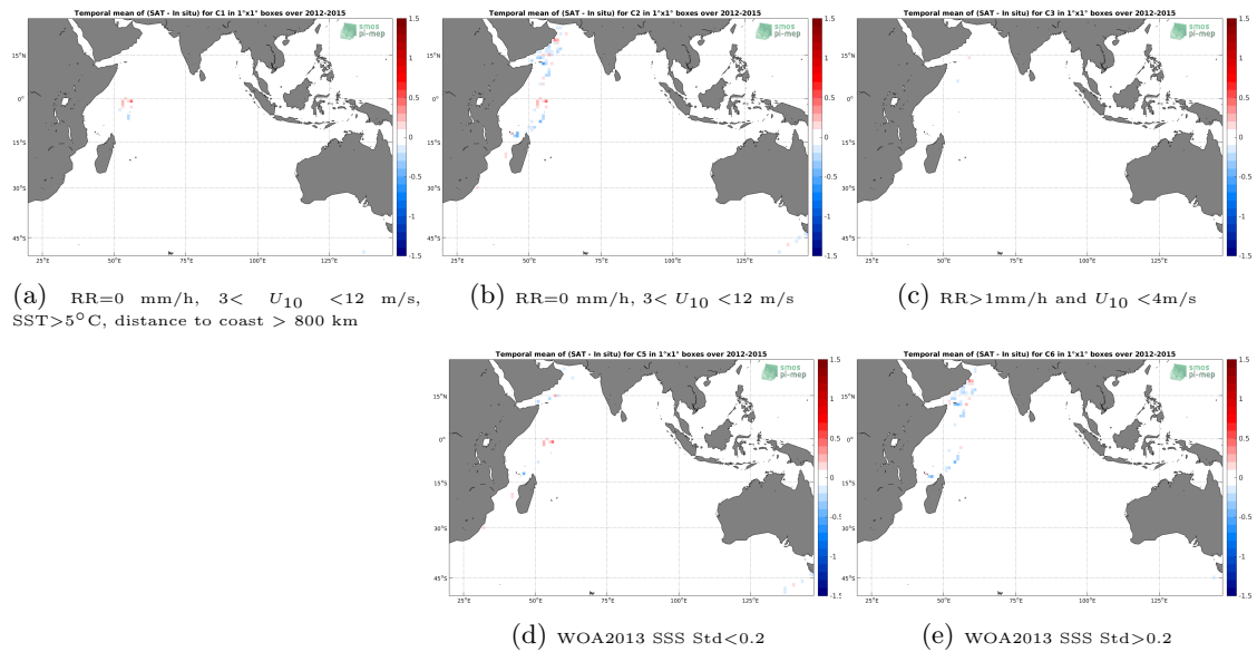
Figure 12: Temporal mean gridded over spatial boxes of size 1^\circ \times 1^\circ of \Delta SSS (Aquarius-L4-IPRC-V5-WEEKLY - TSG-GOSUD-Research-vessel) for 5 different subdatasets corresponding to:RR=0 mm/h, 3 < U_{10} < 12 m/s, SST >5^\circ C, distance to coast > 800 km (a), RR=0 mm/h, 3 < U_{10} < 12 m/s (b), RR >1 mm/h and U_{10} < 4 m/s (c), WOA2013 SSS Std <0.2 (d), WOA2013 SSS Std >0.2 (e).
