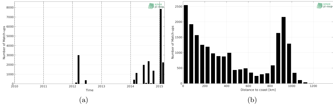
Figure 1: Number of match-ups between TSG-GOSUD-Research-vessel and Aquarius-L4-IPRC-V5-WEEKLY SSS as a function of time (a) and as function of the distance to coast (b) over the Indian Ocean Pi-MEP region and for the full satellite product period.
