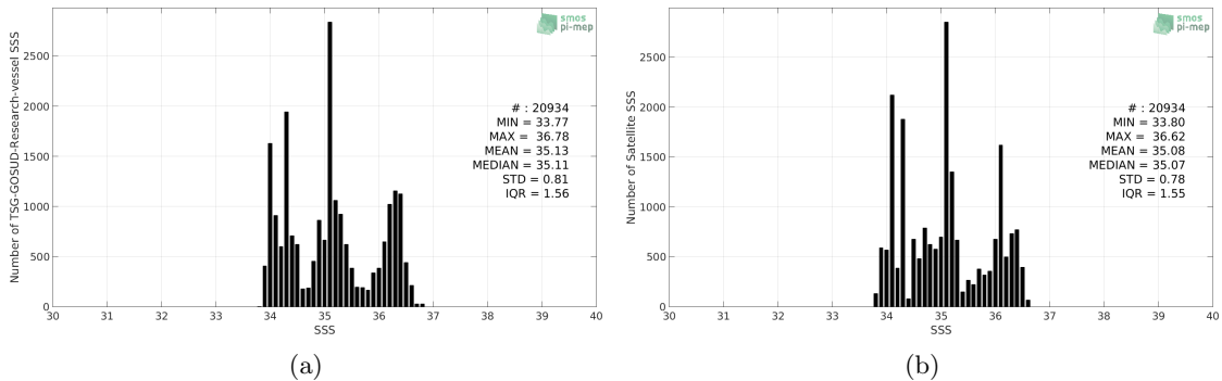
Figure 2: Histograms of SSS from TSG-GOSUD-Research-vessel (a) and Aquarius-L4-IPRC-V5-WEEKLY (b) considering all match-up pairs per bins of 0.1 over the Indian Ocean Pi-MEP region and for the full satellite product period.
