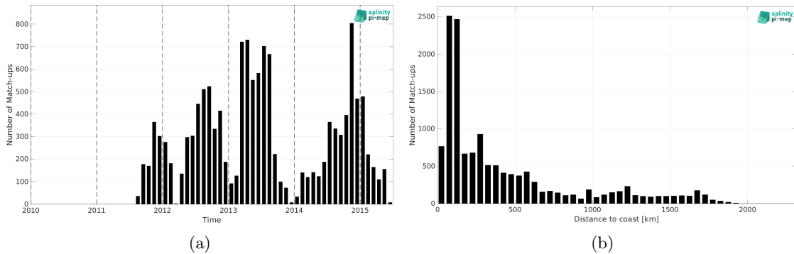
Figure 2: Number of match-ups between Marine mammals and Aquarius SSS L4 OI v5 - Weekly (IPRC) SSS as a function of time (a) and as function of the distance to coast (b) over the Indian Ocean Pi-MEP region and for the full satellite product period.
