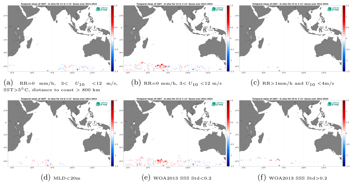
Figure 14: Temporal mean gridded over spatial boxes of size 1^\circ \times 1^\circ of \Delta SSS (Aquarius SSS L4 OI v5 - Weekly (IPRC) - Marine mammals) for 6 different subdatasets corresponding to:RR=0 mm/h, 3 < U_{10} < 12 m/s, SST > 5^\circ\text{C} , distance to coast > 800 km (a), RR=0 mm/h, 3 < U_{10} < 12 m/s (b), RR > 1 mm/h and U_{10} < 4 m/s (c),MLD < 20 m (d),WOA2013 SSS Std < 0.2 (e),WOA2013 SSS Std > 0.2 (f).
