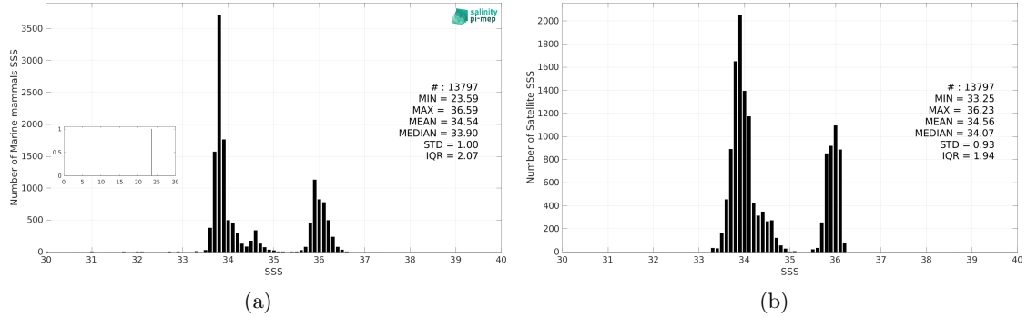
Figure 3: Histograms of SSS from Marine mammals (a) and Aquarius SSS L4 OI v5 - Weekly (IPRC) (b) considering all match-up pairs per bins of 0.1 over the Indian Ocean Pi-MEP region and for the full satellite product period.
