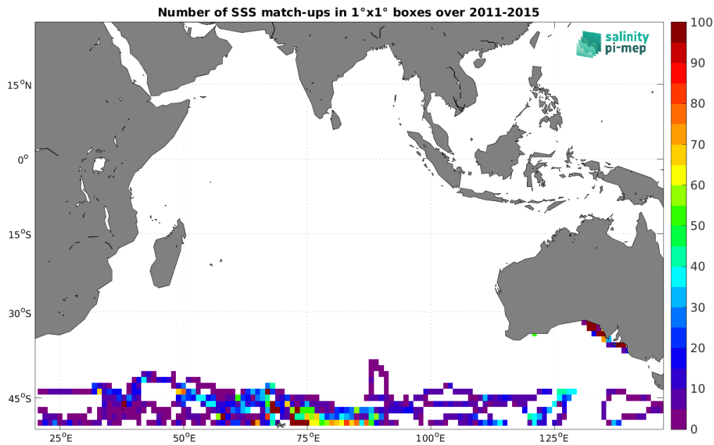
Figure 5: Number of SSS match-ups between Marine mammals SSS and the Aquarius SSS L4 OI v5 - Weekly (IPRC) SSS product for the Indian Ocean Pi-MEP region over 1^\circ \times 1^\circ boxes and for the full satellite product period.
