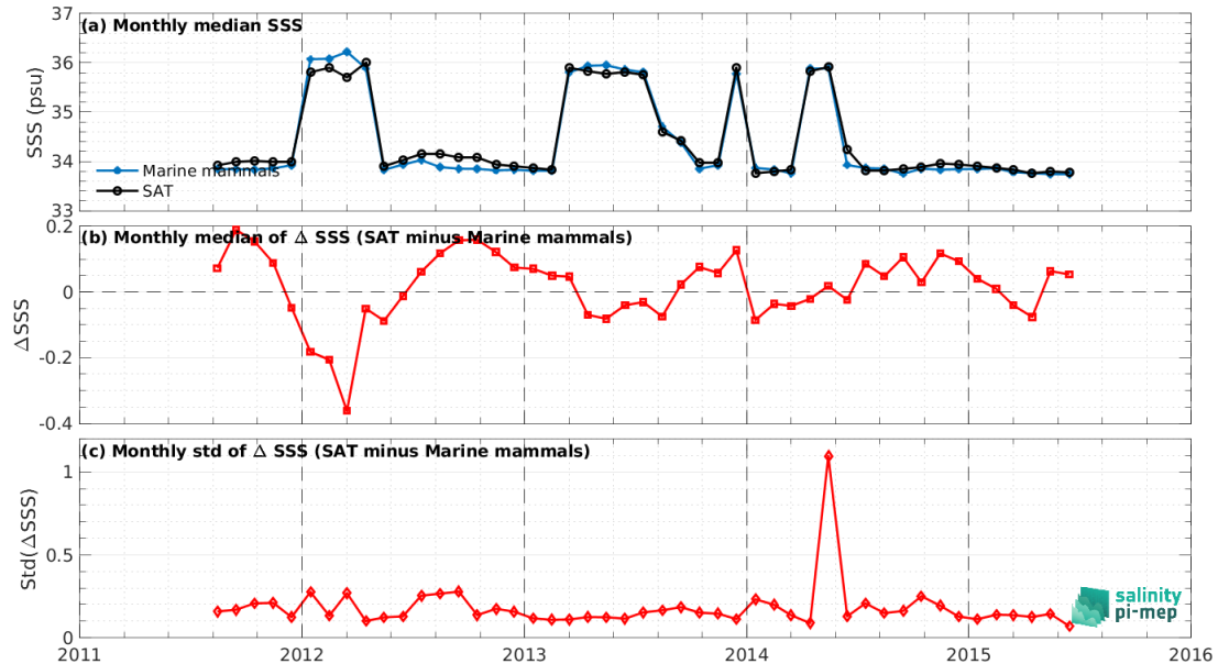
Figure 8: Time series of the monthly median SSS (top), median of \Delta\text{SSS} (Satellite - Marine mammals) and Std of \Delta\text{SSS} (Satellite - Marine mammals) over the Indian Ocean Pi-MEP region considering all match-ups collected by the Pi-MEP.
