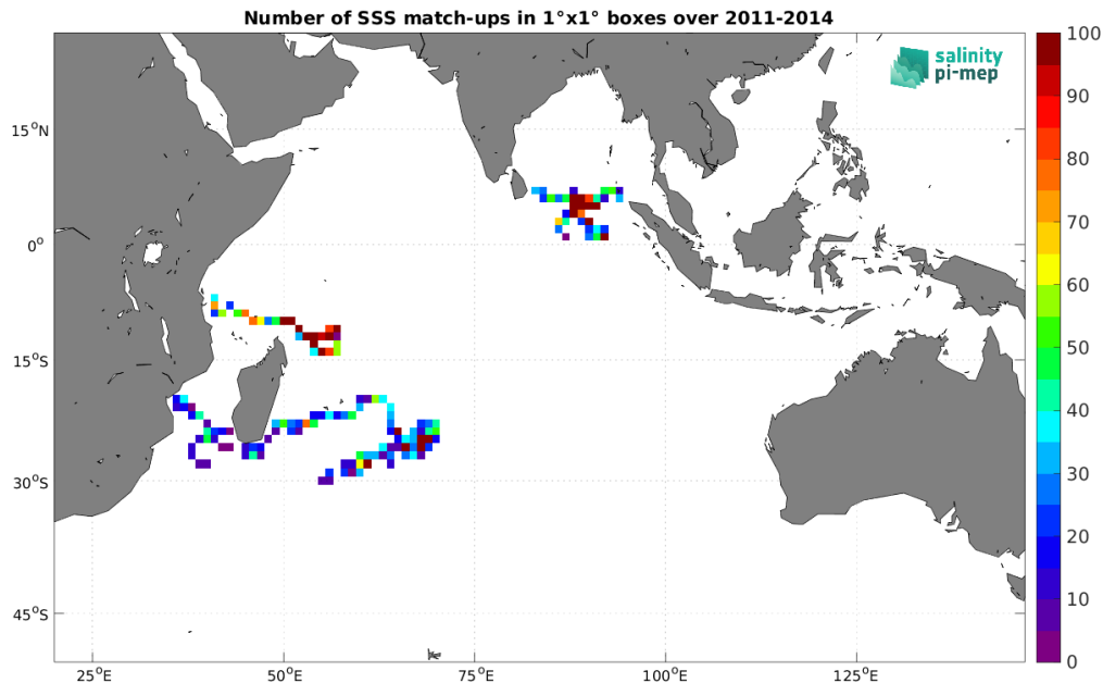
Figure 4: Number of SSS match-ups between Surface drifters SSS and the Aquarius SSS L4 OI v5 - Weekly (IPRC) SSS product for the Indian Ocean Pi-MEP region over 1^\circ \times 1^\circ boxes and for the full satellite product period.
