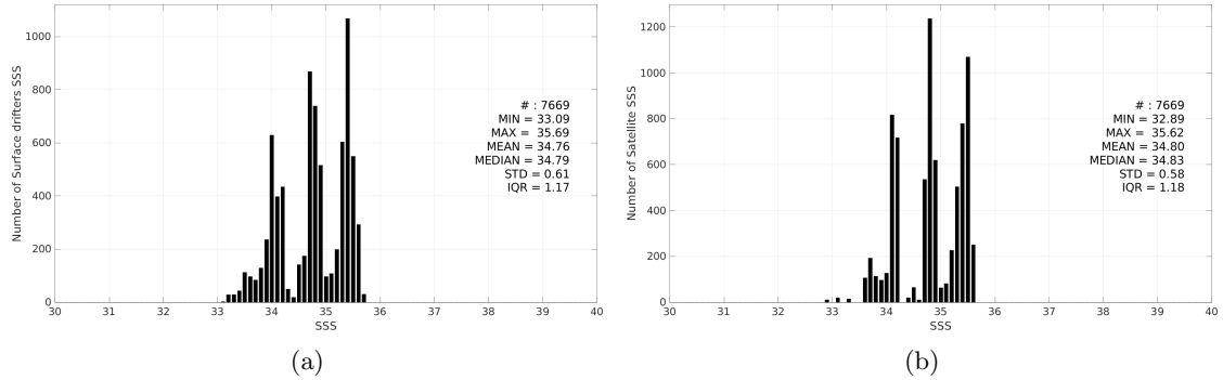
Figure 3: Histograms of SSS from Surface drifters (a) and Aquarius SSS L4 OI v5 - Weekly (IPRC) (b) considering all match-up pairs per bins of 0.1 over the Indian Ocean Pi-MEP region and for the full satellite product period.
