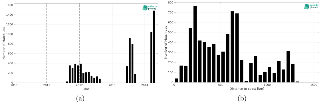
Figure 2: Number of match-ups between Surface drifters and Aquarius SSS L4 OI v5 - Weekly (IPRC) SSS as a function of time (a) and as function of the distance to coast (b) over the Indian Ocean Pi-MEP region and for the full satellite product period.
