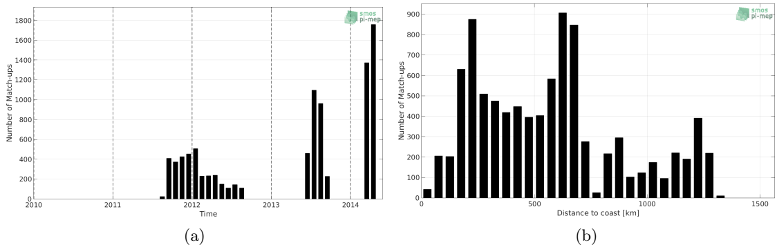
Figure 1: Number of match-ups between Surface drifters and Aquarius-L4-IPRC-V5-WEEKLY SSS as a function of time (a) and as function of the distance to coast (b) over the Indian Ocean Pi-MEP region and for the full satellite product period.
