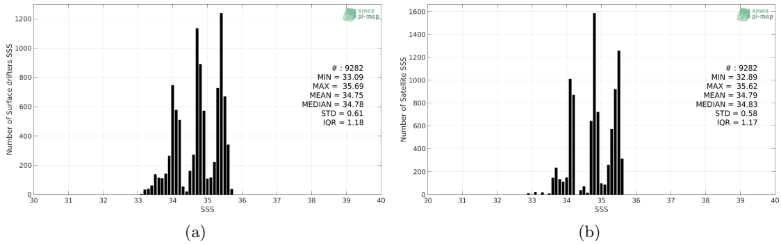
Figure 2: Histograms of SSS from Surface drifters (a) and Aquarius-L4-IPRC-V5-WEEKLY (b) considering all match-up pairs per bins of 0.1 over the Indian Ocean Pi-MEP region and for the full satellite product period.
