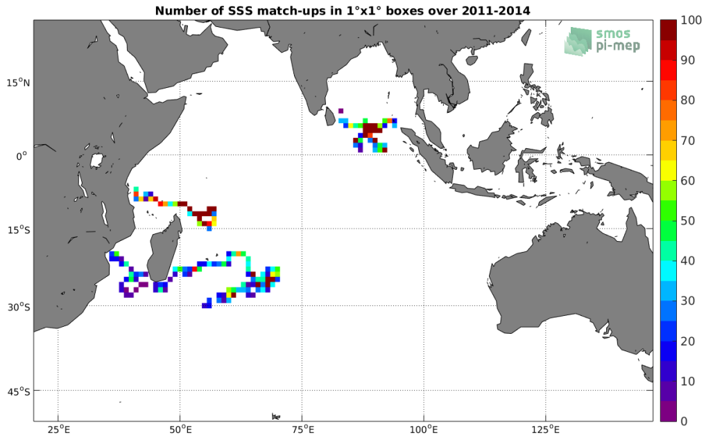
Figure 3: Number of SSS match-ups between Surface drifters SSS and the Aquarius-L4-IPRC-V5-WEEKLY SSS product for the Indian Ocean Pi-MEP region over 1°x1° boxes and for the full satellite product period.
