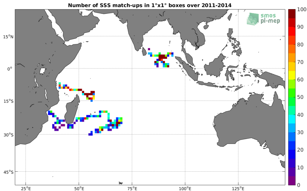
Figure 3: Number of SSS match-ups between Surface drifters SSS and the Aquarius-L4-IPRC-V5-WEEKLY SSS product for the Indian Ocean Pi-MEP region over 1^\circ \times 1^\circ boxes and for the full satellite product period.
