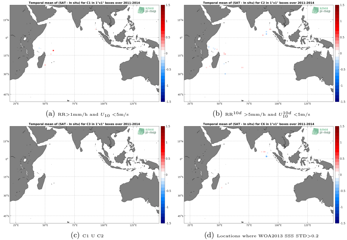
Figure 11: Temporal mean gridded over spatial boxes of size 1^\circ \times 1^\circ of \Delta SSS (Aquarius-L4-IPRC-V5-WEEKLY - Surface drifters) for 4 different subdatasets corresponding to: RR > 1 mm/h and U_{10} < 5 m/s (a), RR 10d > 5 mm/h and U_{10}^{10d} < 5 m/s (b), C1 U C2 (c), Locations where WOA2013 SSS STD > 0.2 (d).
