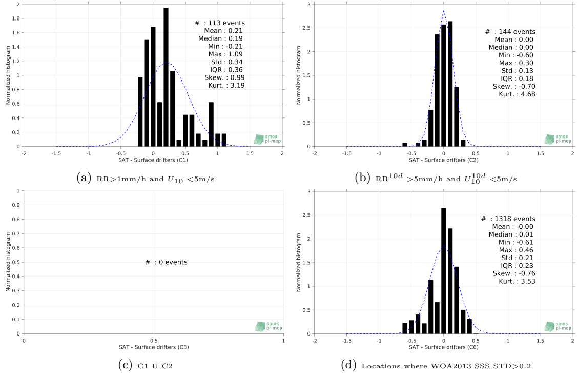
Figure 12: Normalized histogram of \Delta SSS (Aquarius-L4-IPRC-V5-WEEKLY - Surface drifters) for 6 different subdatasets corresponding to: RR > 1\text{mm/h} and U_{10} < 5\text{m/s} (a), RR^{10d} > 5\text{mm/h} and U_{10}^{10d} < 5\text{m/s} (b), C1 \cup C2 (c), Locations where WOA2013 SSS STD > 0.2 (d).
