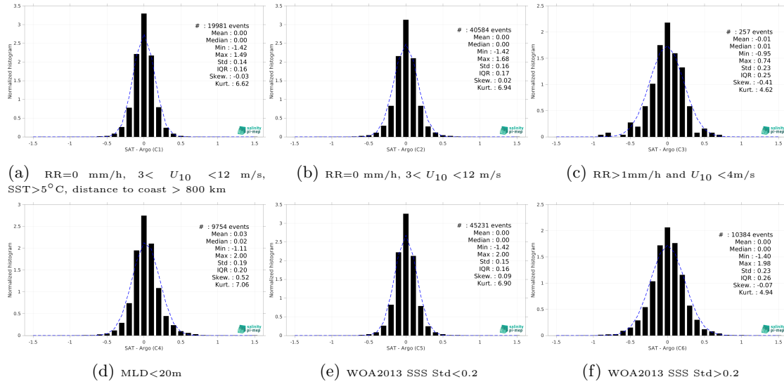
Figure 15: Normalized histogram of \Delta SSS (Aquarius SSS L4 OI v5 - Weekly (IPRC) - Argo) for 6 different subdatasets corresponding to: RR=0 mm/h, 3 < U_{10} < 12 m/s, SST >5^{\circ}\text{C} , distance to coast > 800 km (a), RR=0 mm/h, 3 < U_{10} < 12 m/s (b), RR >1 mm/h and U_{10} < 4 m/s (c), MLD <20 m (d), WOA2013 SSS Std <0.2 (e), WOA2013 SSS Std >0.2 (f).
