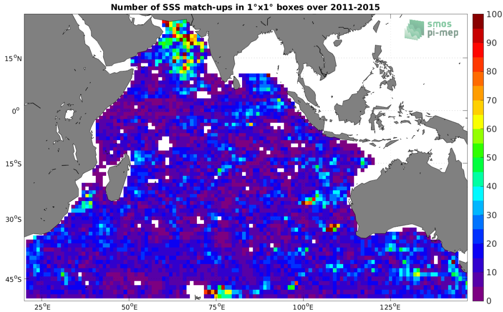
Figure 4: Number of SSS match-ups between Argo SSS and the Aquarius SSS L4 OI v5 - Weekly (IPRC) SSS product for the Indian Ocean Pi-MEP region over 1^\circ \times 1^\circ boxes and for the full satellite product period.
