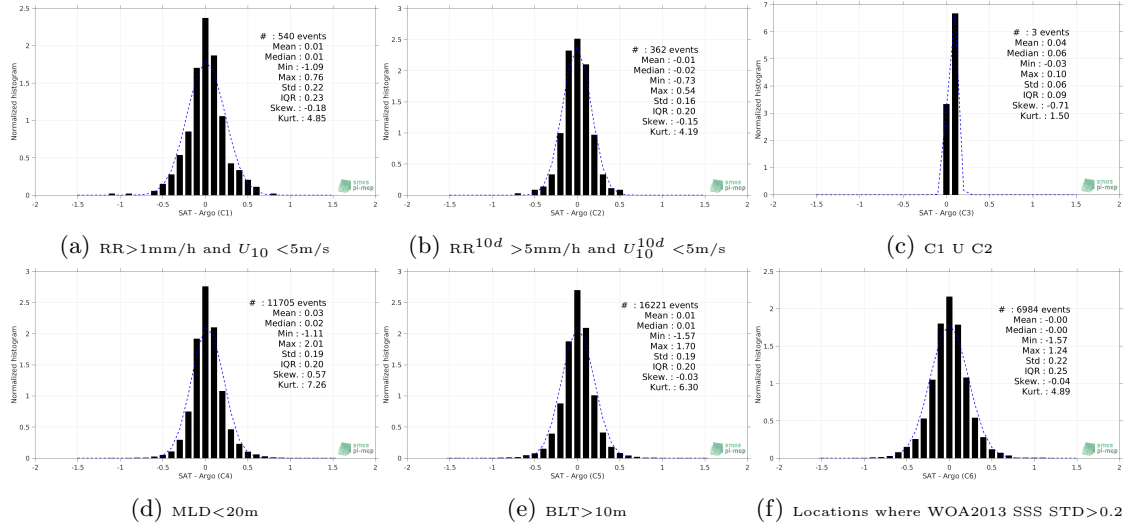
Figure 13: Normalized histogram of \Delta SSS (Aquarius-L4-IPRC-V5-WEEKLY - Argo) for 6 different subdatasets corresponding to: RR > 1\text{mm/h} and U_{10} < 5\text{m/s} (a), RR^{10d} > 5\text{mm/h} and U_{10}^{10d} < 5\text{m/s} (b), C1 U C2 (c), MLD < 20\text{m} (d), BLT > 10\text{m} (e), Locations where WOA2013 SSS STD > 0.2 (f).
