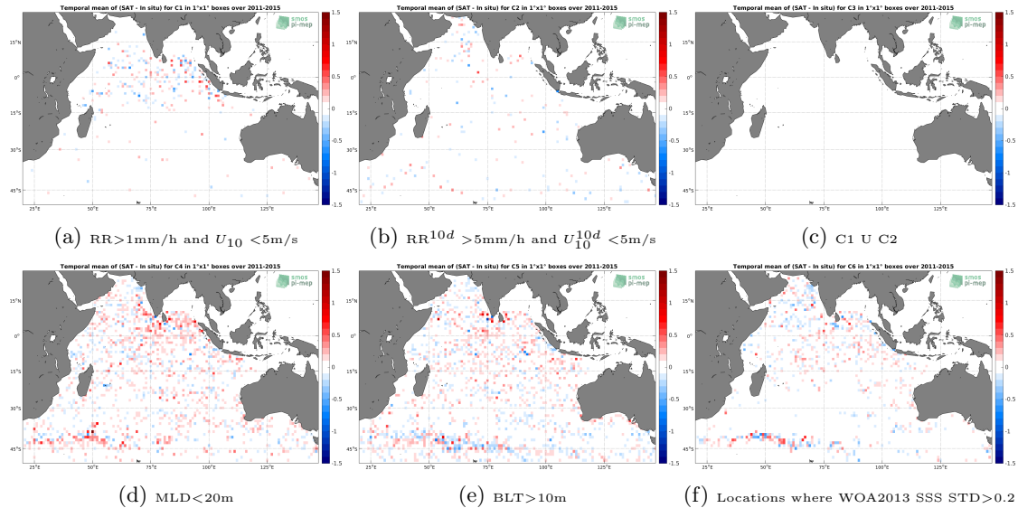
Figure 12: Temporal mean gridded over spatial boxes of size 1^\circ \times 1^\circ of \Delta\text{SSS} (Aquarius-L4-IPRC-V5-WEEKLY - Argo) for 6 different subdatasets corresponding to: RR > 1\text{mm/h} and U_{10} < 5\text{m/s} (a), RR^{10d} > 5\text{mm/h} and U_{10}^{10d} < 5\text{m/s} (b), C1 U C2 (c), MLD < 20\text{m} (d), BLT > 10\text{m} (e), Locations where WOA2013 SSS STD > 0.2 (f).
