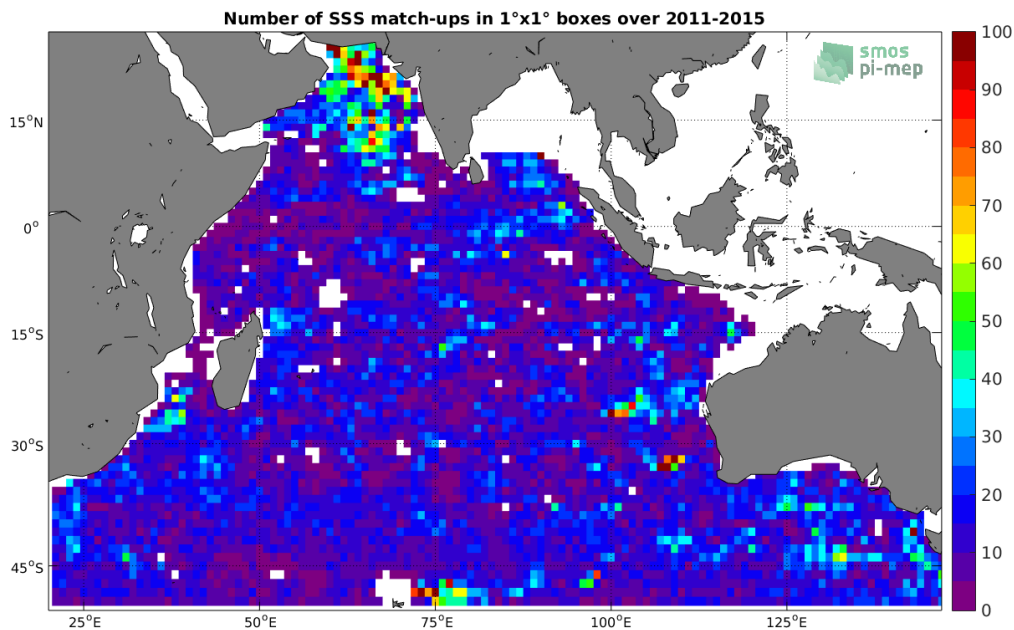
Figure 4: Number of SSS match-ups between Argo SSS and the Aquarius-L4-IPRC-V5-WEEKLY SSS product for the Indian Ocean Pi-MEP region over 1^\circ \times 1^\circ boxes and for the full satellite product period.
