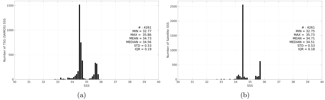
Figure 3: Histograms of SSS from TSG (SAMOS) (a) and Aquarius SSS L4 OI v5 - Monthly (IPRC) (b) considering all match-up pairs per bins of 0.1 over the Indian Ocean Pi-MEP region and for the full satellite product period.
