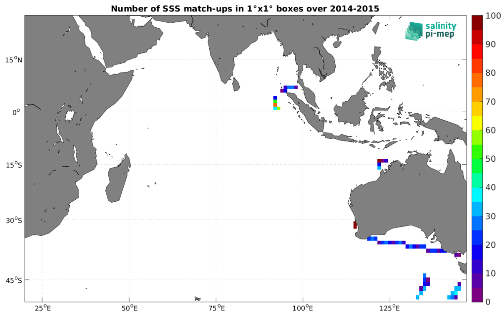
Figure 5: Number of SSS match-ups between TSG (SAMOS) SSS and the Aquarius SSS L4 OI v5 - Monthly (IPRC) SSS product for the Indian Ocean Pi-MEP region over 1^\circ \times 1^\circ boxes and for the full satellite product period.
