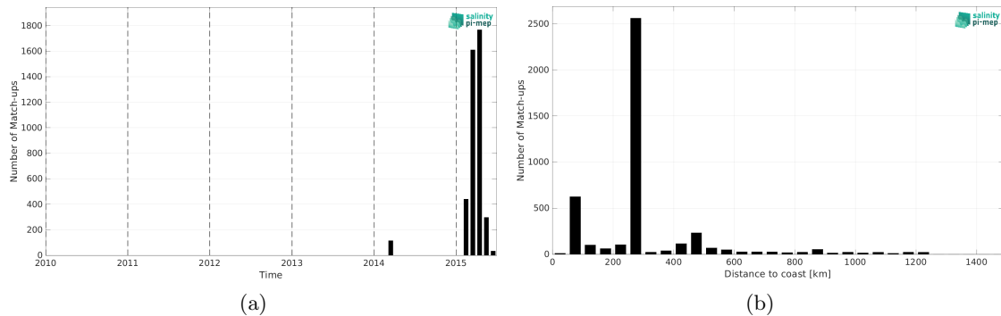
Figure 2: Number of match-ups between TSG (SAMOS) and Aquarius SSS L4 OI v5 - Monthly (IPRC) SSS as a function of time (a) and as function of the distance to coast (b) over the Indian Ocean Pi-MEP region and for the full satellite product period.
