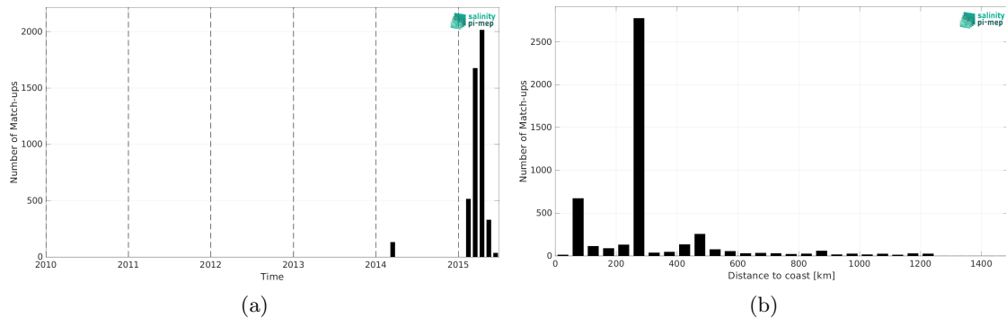
Figure 1: Number of match-ups between TSG (SAMOS) and Aquarius SSS L4 OI v5 - Monthly (IPRC) SSS as a function of time (a) and as function of the distance to coast (b) over the Indian Ocean Pi-MEP region and for the full satellite product period.
