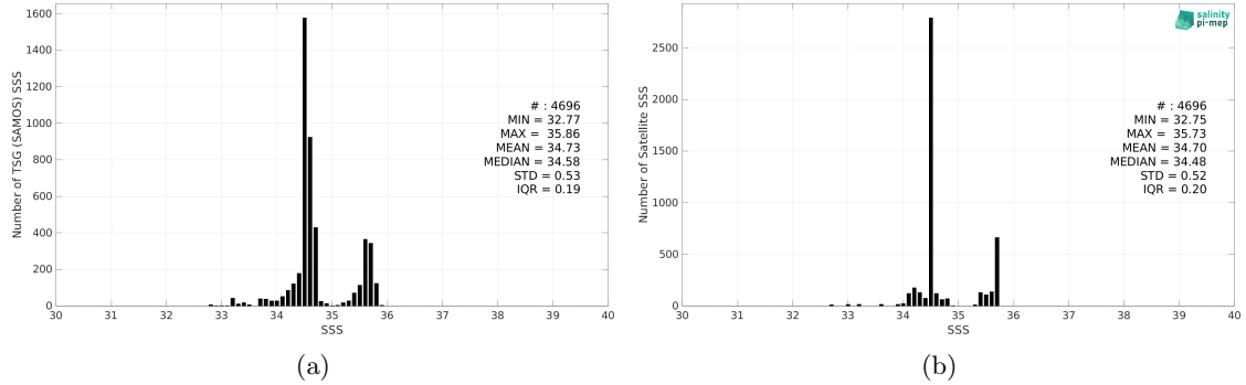
Figure 2: Histograms of SSS from TSG (SAMOS) (a) and Aquarius SSS L4 OI v5 - Monthly (IPRC) (b) considering all match-up pairs per bins of 0.1 over the Indian Ocean Pi-MEP region and for the full satellite product period.
