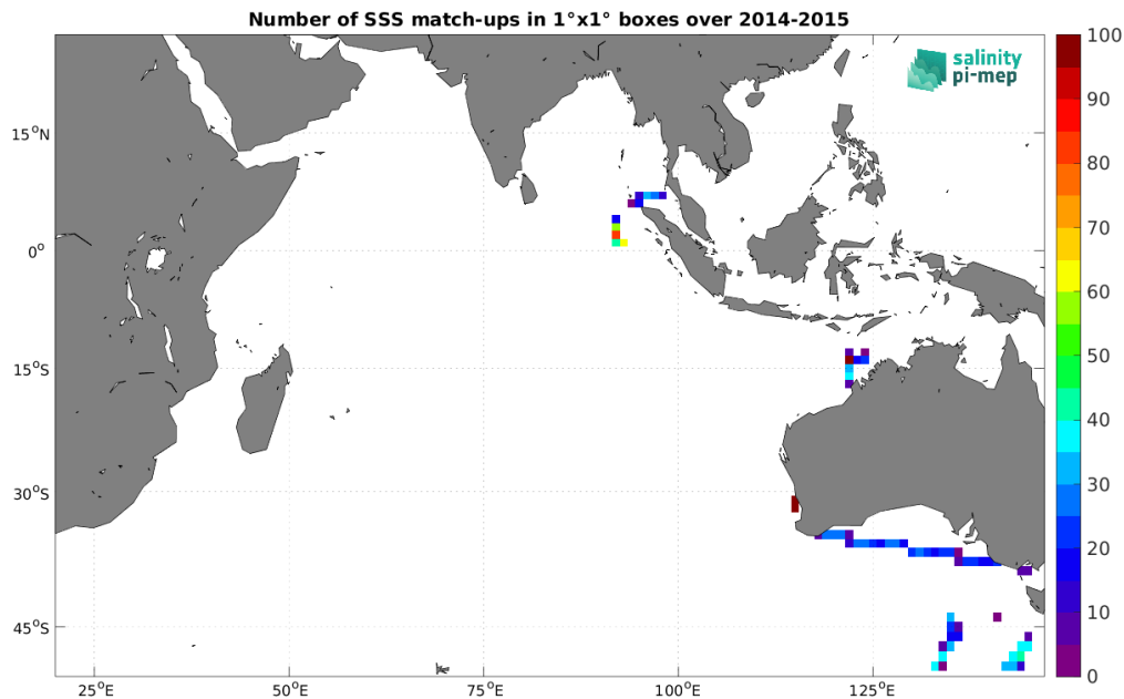
Figure 4: Number of SSS match-ups between TSG (SAMOS) SSS and the Aquarius SSS L4 OI v5 - Monthly (IPRC) SSS product for the Indian Ocean Pi-MEP region over 1^\circ \times 1^\circ boxes and for the full satellite product period.
