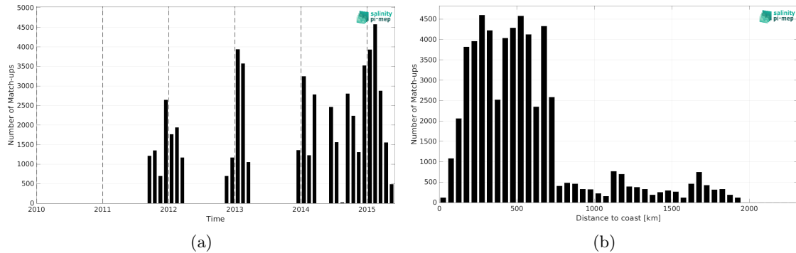
Figure 2: Number of match-ups between TSG (LEGOS-DM) and Aquarius SSS L4 OI v5 - Monthly (IPRC) SSS as a function of time (a) and as function of the distance to coast (b) over the Indian Ocean Pi-MEP region and for the full satellite product period.
