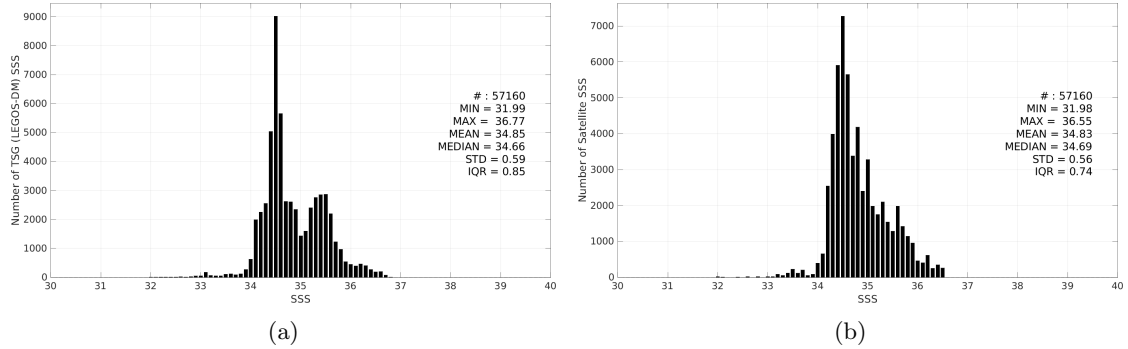
Figure 3: Histograms of SSS from TSG (LEGOS-DM) (a) and Aquarius SSS L4 OI v5 - Monthly (IPRC) (b) considering all match-up pairs per bins of 0.1 over the Indian Ocean Pi-MEP region and for the full satellite product period.
