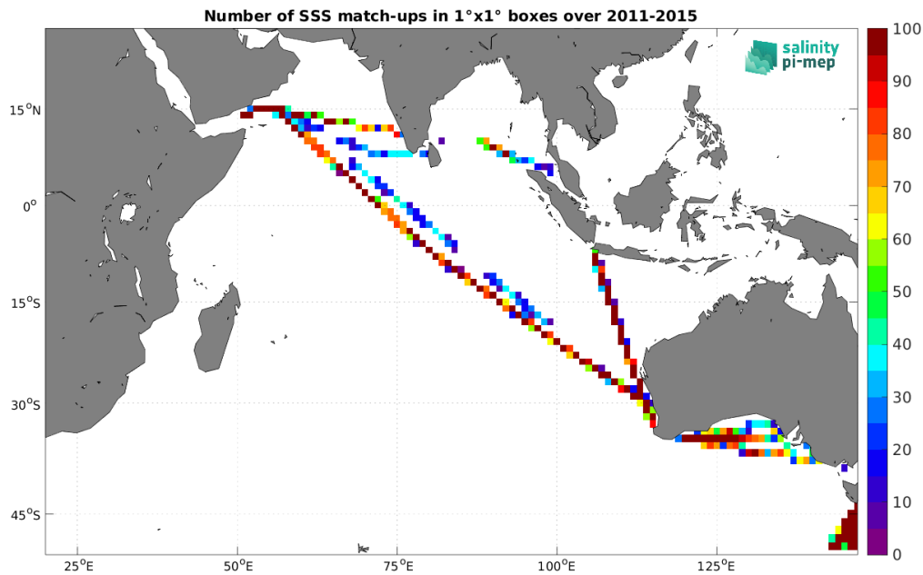
Figure 5: Number of SSS match-ups between TSG (LEGOS-DM) SSS and the Aquarius SSS L4 OI v5 - Monthly (IPRC) SSS product for the Indian Ocean Pi-MEP region over 1^{\circ} \times 1^{\circ} boxes and for the full satellite product period.
