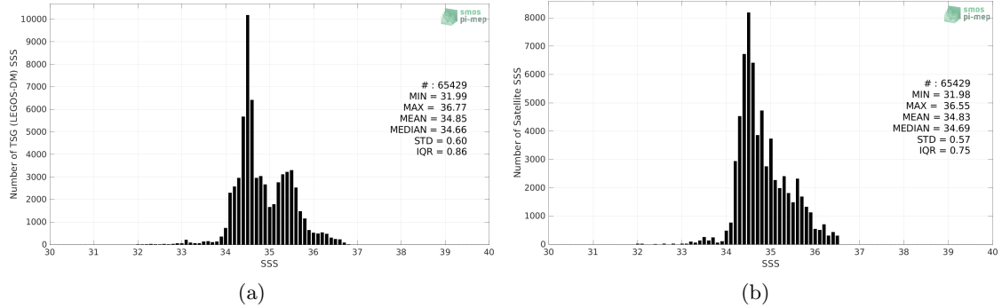
Figure 2: Histograms of SSS from TSG (LEGOS-DM) (a) and Aquarius SSS L4 OI v5 - Monthly (IPRC) (b) considering all match-up pairs per bins of 0.1 over the Indian Ocean Pi-MEP region and for the full satellite product period.
