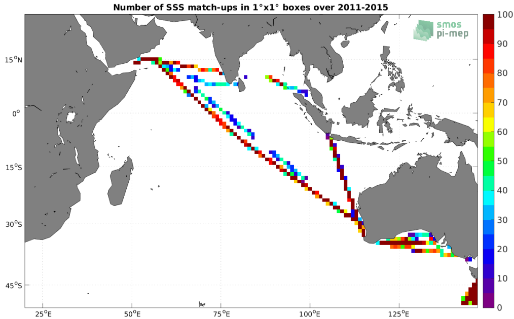
Figure 4: Number of SSS match-ups between TSG (LEGOS-DM) SSS and the Aquarius SSS L4 OI v5 - Monthly (IPRC) SSS product for the Indian Ocean Pi-MEP region over 1^\circ \times 1^\circ boxes and for the full satellite product period.
