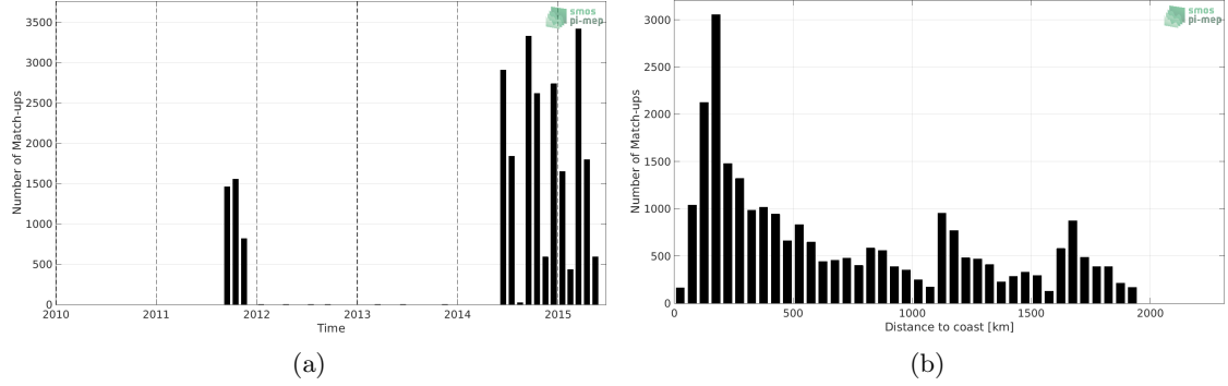
Figure 1: Number of match-ups between TSG (LEGOS-DM) and Aquarius SSS L4 OI v5 - Monthly (IPRC) SSS as a function of time (a) and as function of the distance to coast (b) over the Indian Ocean Pi-MEP region and for the full satellite product period.
