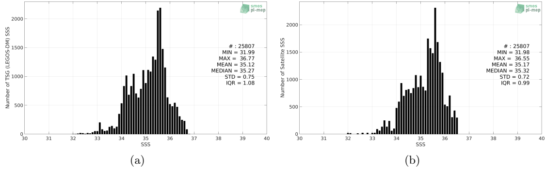
Figure 2: Histograms of SSS from TSG (LEGOS-DM) (a) and Aquarius SSS L4 OI v5 - Monthly (IPRC) (b) considering all match-up pairs per bins of 0.1 over the Indian Ocean Pi-MEP region and for the full satellite product period.
