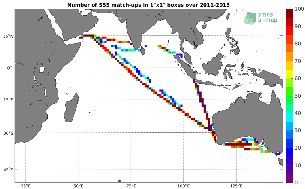
Figure 4: Number of SSS match-ups between TSG-LEGOS-DM SSS and the Aquarius-L4-IPRC-V5-MONTHLY SSS product for the Indian Ocean Pi-MEP region over 1°x1° boxes and for the full satellite product period.
