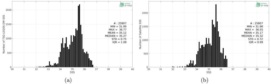
Figure 2: Histograms of SSS from TSG-LEGOS-DM (a) and Aquarius-L4-IPRC-V5-MONTHLY (b) considering all match-up pairs per bins of 0.1 over the Indian Ocean Pi-MEP region and for the full satellite product period.
