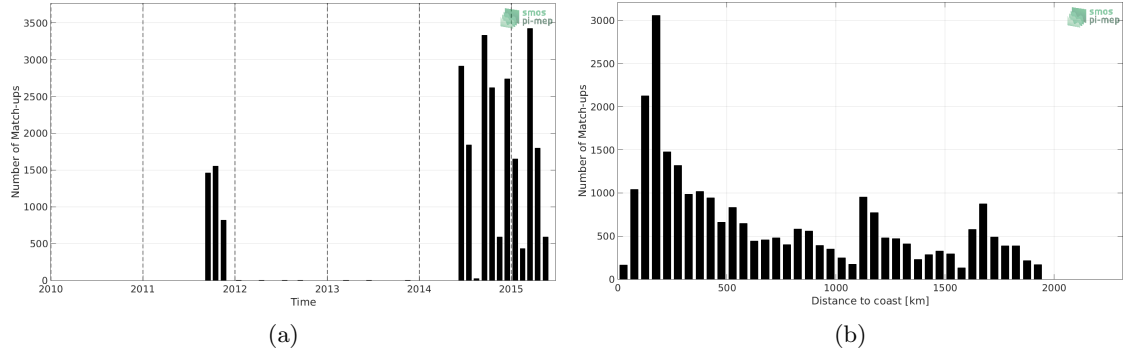
Figure 1: Number of match-ups between TSG-LEGOS-DM and Aquarius-L4-IPRC-V5-MONTHLY SSS as a function of time (a) and as function of the distance to coast (b) over the Indian Ocean Pi-MEP region and for the full satellite product period.
