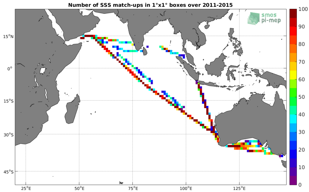
Figure 4: Number of SSS match-ups between TSG-LEGOS-DM SSS and the Aquarius-L4-IPRC-V5-MONTHLY SSS product for the Indian Ocean Pi-MEP region over 1^\circ \times 1^\circ boxes and for the full satellite product period.
