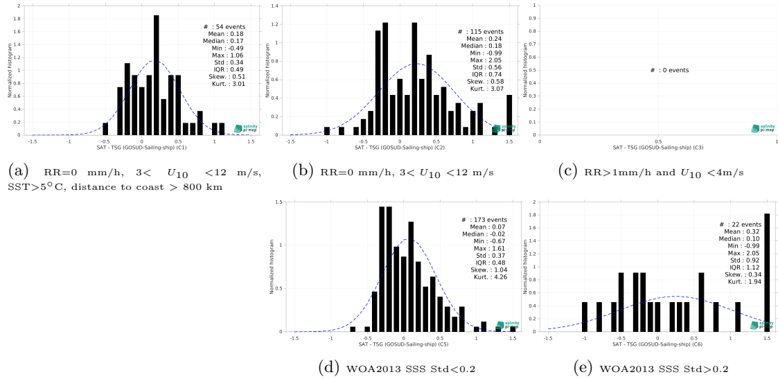
Figure 15: Normalized histogram of \Delta SSS (Aquarius SSS L4 OI v5 - Monthly (IPRC) - TSG (GOSUD-Sailing-ship)) for 5 different subdatasets corresponding to: RR=0 mm/h, 3 < U_{10} < 12 m/s, SST > 5°C, distance to coast > 800 km (a), RR=0 mm/h, 3 < U_{10} < 12 m/s (b), RR > 1mm/h and U_{10} < 4 m/s (c), WOA2013 SSS Std < 0.2 (d), WOA2013 SSS Std > 0.2 (e).
