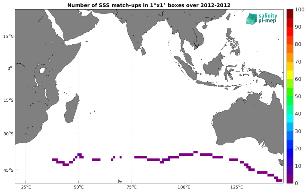
Figure 5: Number of SSS match-ups between TSG (GOSUD-Sailing-ship) SSS and the Aquarius SSS L4 OI v5 - Monthly (IPRC) SSS product for the Indian Ocean Pi-MEP region over 1^\circ \times 1^\circ boxes and for the full satellite product period.
