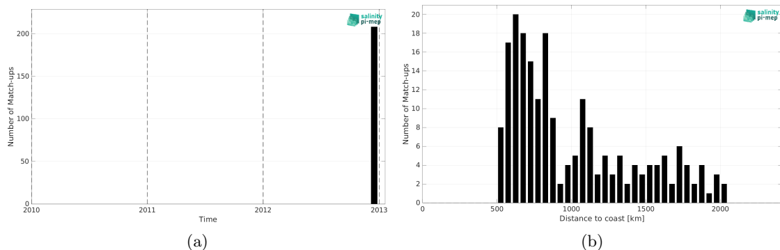
Figure 2: Number of match-ups between TSG (GOSUD-Sailing-ship) and Aquarius SSS L4 OI v5 - Monthly (IPRC) SSS as a function of time (a) and as function of the distance to coast (b) over the Indian Ocean Pi-MEP region and for the full satellite product period.
