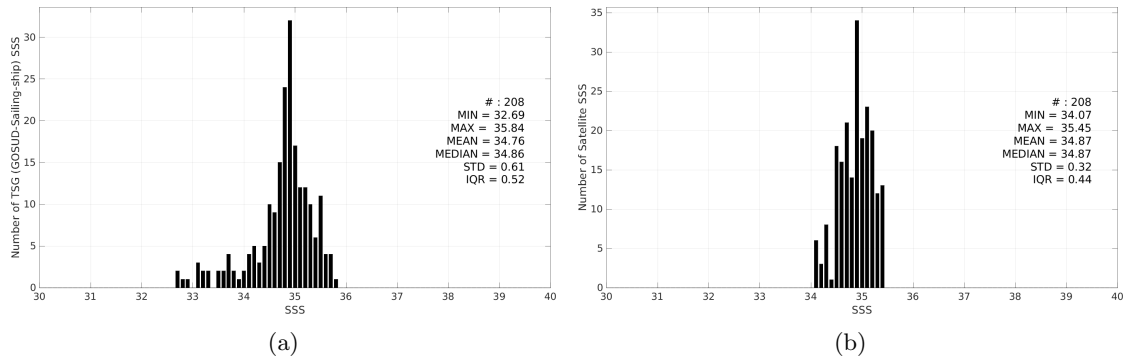
Figure 3: Histograms of SSS from TSG (GOSUD-Sailing-ship) (a) and Aquarius SSS L4 OI v5 - Monthly (IPRC) (b) considering all match-up pairs per bins of 0.1 over the Indian Ocean Pi-MEP region and for the full satellite product period.
