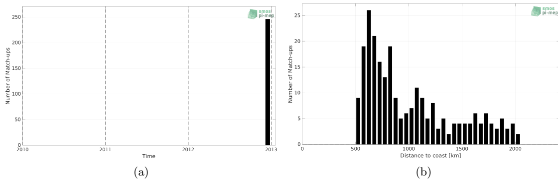
Figure 1: Number of match-ups between TSG (GOSUD-Sailing-ship) and Aquarius SSS L4 OI v5 - Monthly (IPRC) SSS as a function of time (a) and as function of the distance to coast (b) over the Indian Ocean Pi-MEP region and for the full satellite product period.
