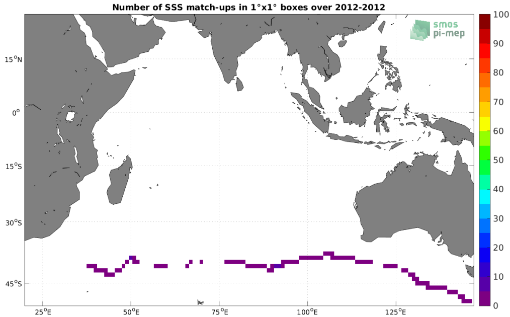
Figure 4: Number of SSS match-ups between TSG (GOSUD-Sailing-ship) SSS and the Aquarius SSS L4 OI v5 - Monthly (IPRC) SSS product for the Indian Ocean Pi-MEP region over 1^\circ \times 1^\circ boxes and for the full satellite product period.
