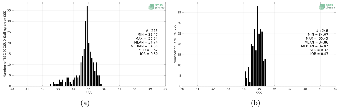
Figure 2: Histograms of SSS from TSG (GOSUD-Sailing-ship) (a) and Aquarius SSS L4 OI v5 - Monthly (IPRC) (b) considering all match-up pairs per bins of 0.1 over the Indian Ocean Pi-MEP region and for the full satellite product period.
