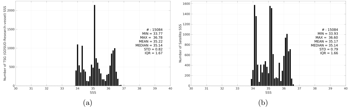
Figure 3: Histograms of SSS from TSG (GOSUD-Research-vessel) (a) and Aquarius SSS L4 OI v5 - Monthly (IPRC) (b) considering all match-up pairs per bins of 0.1 over the Indian Ocean Pi-MEP region and for the full satellite product period.
