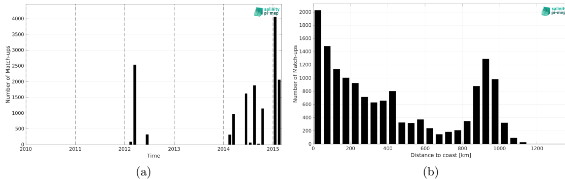
Figure 2: Number of match-ups between TSG (GOSUD-Research-vessel) and Aquarius SSS L4 OI v5 - Monthly (IPRC) SSS as a function of time (a) and as function of the distance to coast (b) over the Indian Ocean Pi-MEP region and for the full satellite product period.
