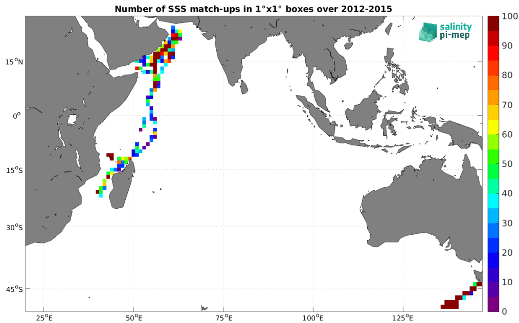
Figure 5: Number of SSS match-ups between TSG (GOSUD-Research-vessel) SSS and the Aquarius SSS L4 OI v5 - Monthly (IPRC) SSS product for the Indian Ocean Pi-MEP region over 1^\circ \times 1^\circ boxes and for the full satellite product period.
