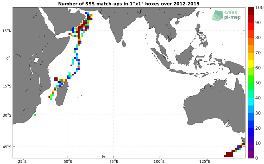
Figure 4: Number of SSS match-ups between TSG (GOSUD-Research-vessel) SSS and the Aquarius SSS L4 OI v5 - Monthly (IPRC) SSS product for the Indian Ocean Pi-MEP region over 1^\circ \times 1^\circ boxes and for the full satellite product period.
