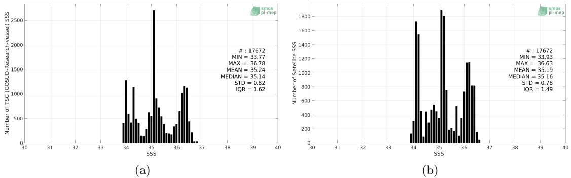
Figure 2: Histograms of SSS from TSG (GOSUD-Research-vessel) (a) and Aquarius SSS L4 OI v5 - Monthly (IPRC) (b) considering all match-up pairs per bins of 0.1 over the Indian Ocean Pi-MEP region and for the full satellite product period.
