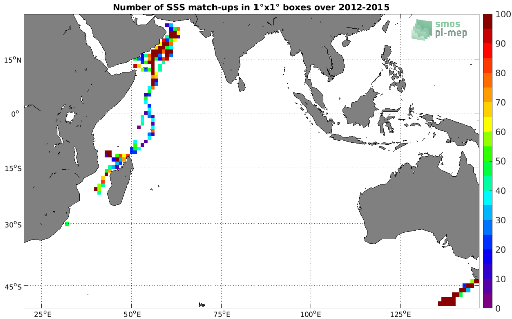
Figure 4: Number of SSS match-ups between TSG (GOSUD-Research-vessel) SSS and the Aquarius SSS L4 OI v5 - Monthly (IPRC) SSS product for the Indian Ocean Pi-MEP region over 1^\circ \times 1^\circ boxes and for the full satellite product period.
