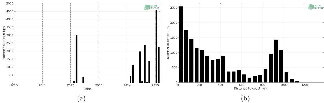
Figure 1: Number of match-ups between TSG (GOSUD-Research-vessel) and Aquarius SSS L4 OI v5 - Monthly (IPRC) SSS as a function of time (a) and as function of the distance to coast (b) over the Indian Ocean Pi-MEP region and for the full satellite product period.
