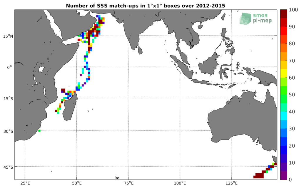
Figure 4: Number of SSS match-ups between TSG-GOSUD-Research-vessel SSS and the Aquarius-L4-IPRC-V5-MONTHLY SSS product for the Indian Ocean Pi-MEP region over 1°x1° boxes and for the full satellite product period.
