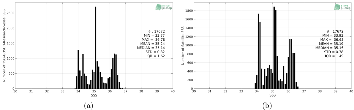
Figure 2: Histograms of SSS from TSG-GOSUD-Research-vessel (a) and Aquarius-L4-IPRC-V5-MONTHLY (b) considering all match-up pairs per bins of 0.1 over the Indian Ocean Pi-MEP region and for the full satellite product period.
