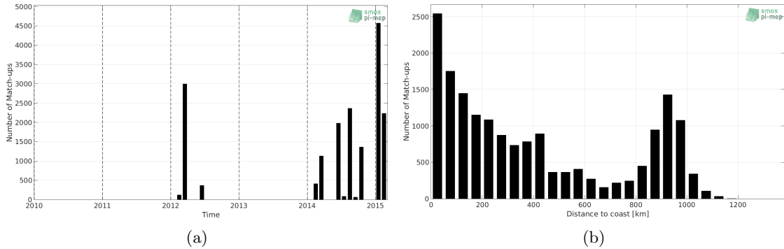
Figure 1: Number of match-ups between TSG-GOSUD-Research-vessel and Aquarius-L4-IPRC-V5-MONTHLY SSS as a function of time (a) and as function of the distance to coast (b) over the Indian Ocean Pi-MEP region and for the full satellite product period.
