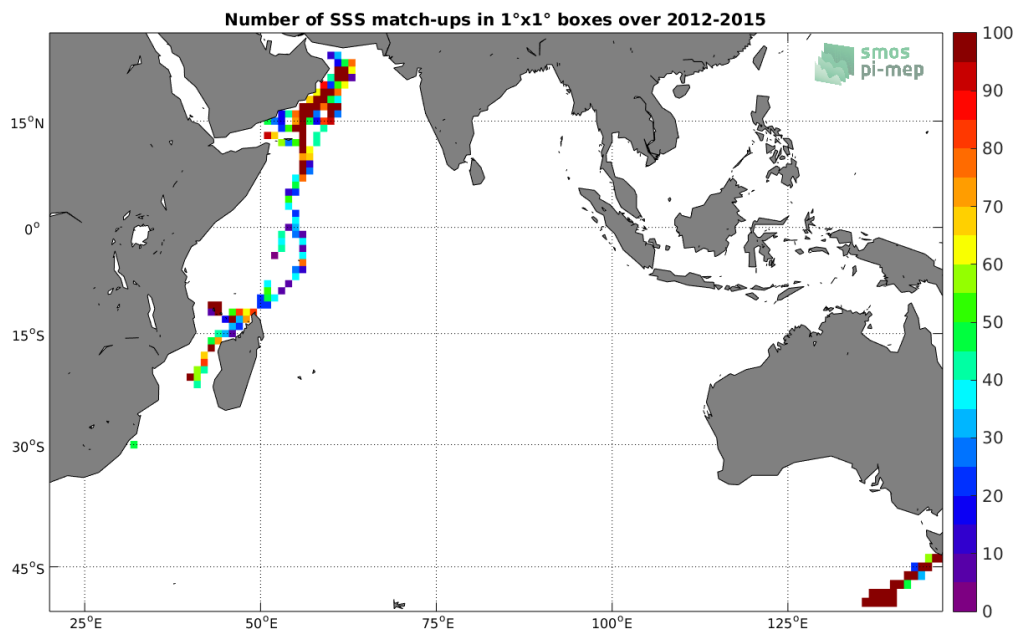
Figure 4: Number of SSS match-ups between TSG-GOSUD-Research-vessel SSS and the Aquarius-L4-IPRC-V5-MONTHLY SSS product for the Indian Ocean Pi-MEP region over 1^\circ \times 1^\circ boxes and for the full satellite product period.
