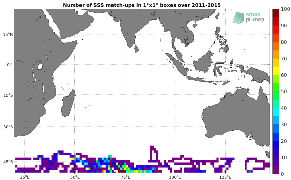
Figure 4: Number of SSS match-ups between Sea mammals SSS and the Aquarius SSS L4 OI v5 - Monthly (IPRC) SSS product for the Indian Ocean Pi-MEP region over 1°x1° boxes and for the full satellite product period.
