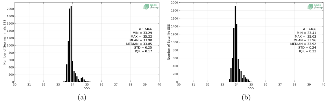
Figure 2: Histograms of SSS from Sea mammals (a) and Aquarius SSS L4 OI v5 - Monthly (IPRC) (b) considering all match-up pairs per bins of 0.1 over the Indian Ocean Pi-MEP region and for the full satellite product period.
