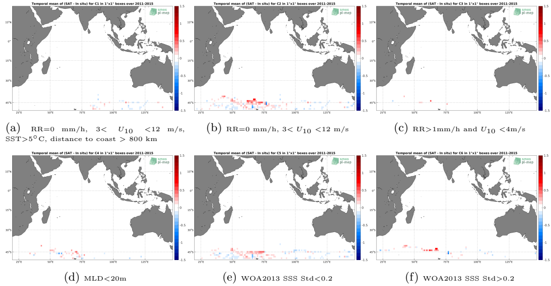
Figure 12: Temporal mean gridded over spatial boxes of size 1^{\circ}\times 1^{\circ} of \Delta\text{SSS} (Aquarius SSS L4 OI v5 - Monthly (IPRC) - Sea mammals) for 6 different subdatasets corresponding to: \text{RR}=0 mm/h, 3 < U_{10} < 12 m/s, \text{SST} > 5^{\circ}\text{C} , distance to coast > 800 km (a), \text{RR}=0 mm/h, 3 < U_{10} < 12 m/s (b), \text{RR} > 1\text{mm/h} and U_{10} < 4\text{m/s} (c), \text{MLD} < 20\text{m} (d), \text{WOA2013 SSS Std} < 0.2 (e), \text{WOA2013 SSS Std} > 0.2 (f).
