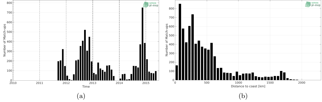
Figure 1: Number of match-ups between Sea mammals and Aquarius SSS L4 OI v5 - Monthly (IPRC) SSS as a function of time (a) and as function of the distance to coast (b) over the Indian Ocean Pi-MEP region and for the full satellite product period.
