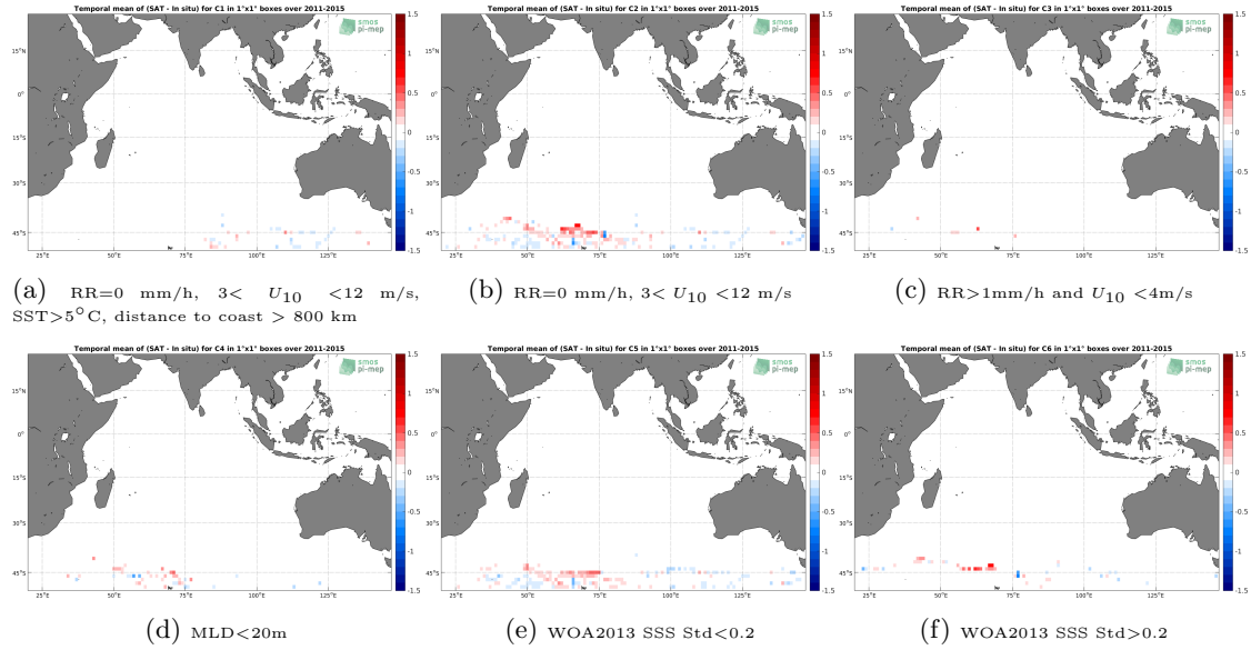
Figure 12: Temporal mean gridded over spatial boxes of size 1^{\circ}\times 1^{\circ} of \Delta\text{SSS} (Aquarius-L4-IPRC-V5-MONTHLY - Sea mammals) for 6 different subdatasets corresponding to: \text{RR}=0 mm/h, 3 < U_{10} < 12 m/s, \text{SST} > 5^{\circ}\text{C} , distance to coast > 800 km (a), \text{RR}=0 mm/h, 3 < U_{10} < 12 m/s (b), \text{RR} > 1\text{mm/h} and U_{10} < 4\text{m/s} (c), \text{MLD} < 20\text{m} (d), \text{WOA2013 SSS Std} < 0.2 (e), \text{WOA2013 SSS Std} > 0.2 (f).
