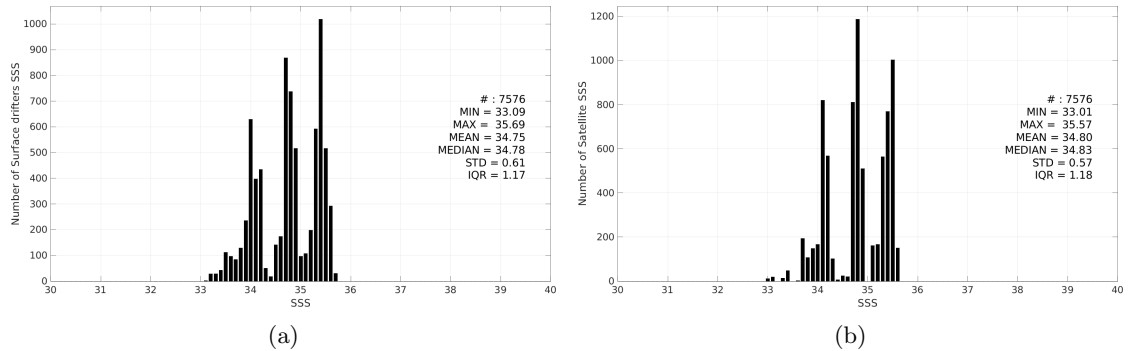
Figure 3: Histograms of SSS from Surface drifters (a) and Aquarius SSS L4 OI v5 - Monthly (IPRC) (b) considering all match-up pairs per bins of 0.1 over the Indian Ocean Pi-MEP region and for the full satellite product period.
