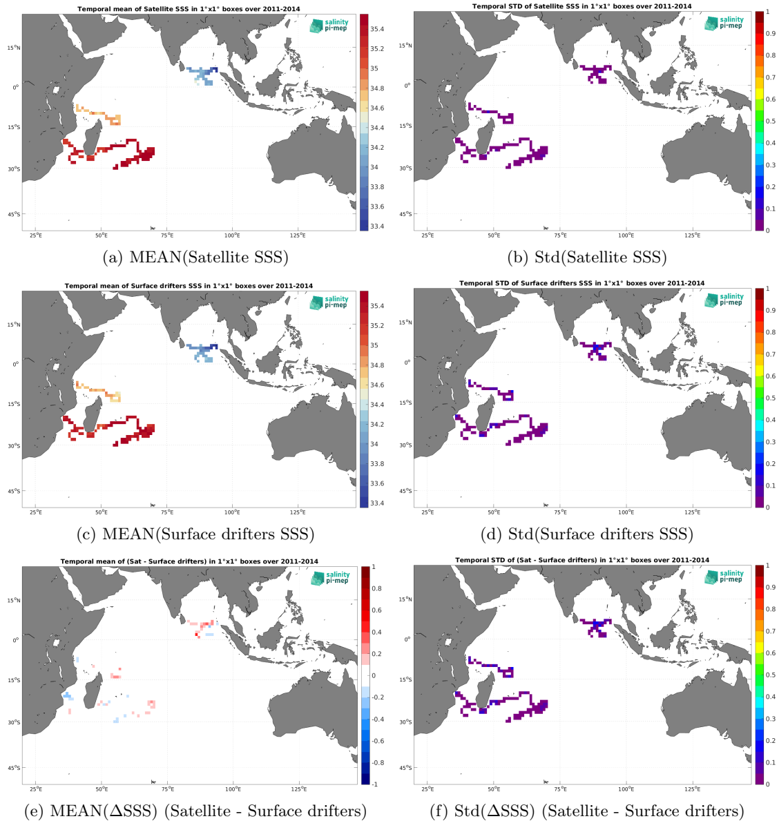
Figure 6: Temporal mean (left) and Std (right) of SSS from Aquarius SSS L4 OI v5 - Monthly (IPRC) (top), Surface drifters (middle), and of \Delta SSS (Satellite - Surface drifters). Only match-up pairs are used to generate these maps.
