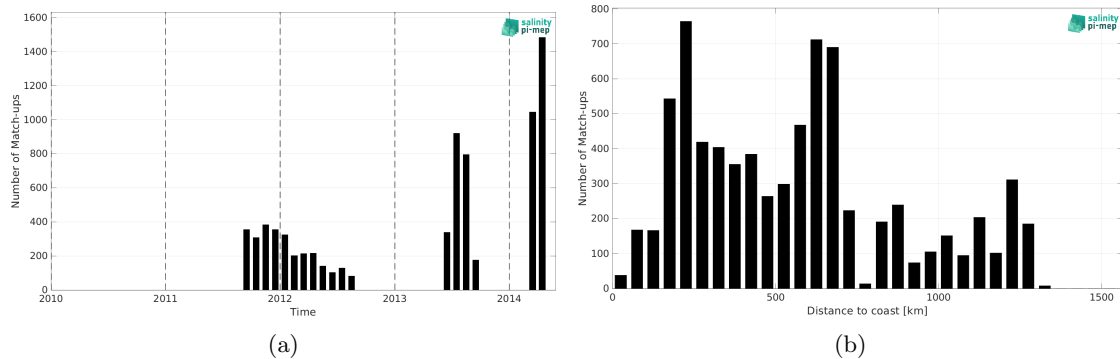
Figure 2: Number of match-ups between Surface drifters and Aquarius SSS L4 OI v5 - Monthly (IPRC) SSS as a function of time (a) and as function of the distance to coast (b) over the Indian Ocean Pi-MEP region and for the full satellite product period.
