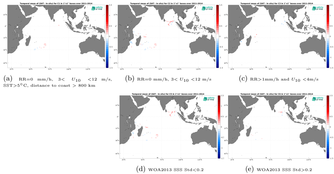
Figure 13: Temporal mean gridded over spatial boxes of size 1^\circ \times 1^\circ of \Delta SSS (Aquarius SSS L4 OI v5 - Monthly (IPRC) - Surface drifters) for 5 different subdatasets corresponding to:RR=0 mm/h, 3 < U_{10} < 12 m/s, SST >5^\circ\text{C} , distance to coast > 800 km (a), RR=0 mm/h, 3 < U_{10} < 12 m/s (b), RR >1 mm/h and U_{10} < 4 m/s (c), WOA2013 SSS Std <0.2 (d), WOA2013 SSS Std >0.2 (e).
