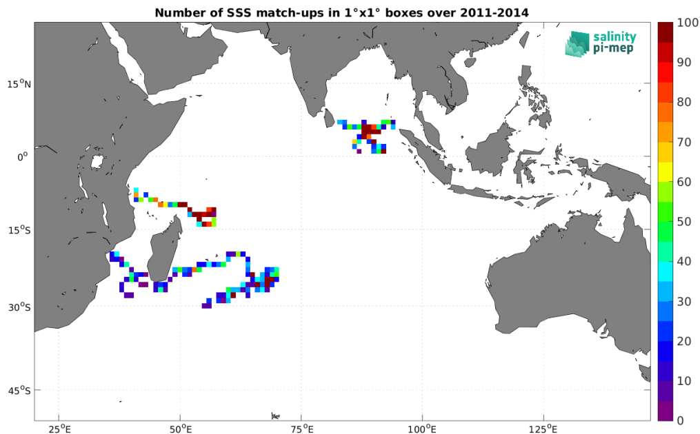
Figure 4: Number of SSS match-ups between Surface drifters SSS and the Aquarius SSS L4 OI v5 - Monthly (IPRC) SSS product for the Indian Ocean Pi-MEP region over 1^\circ \times 1^\circ boxes and for the full satellite product period.
