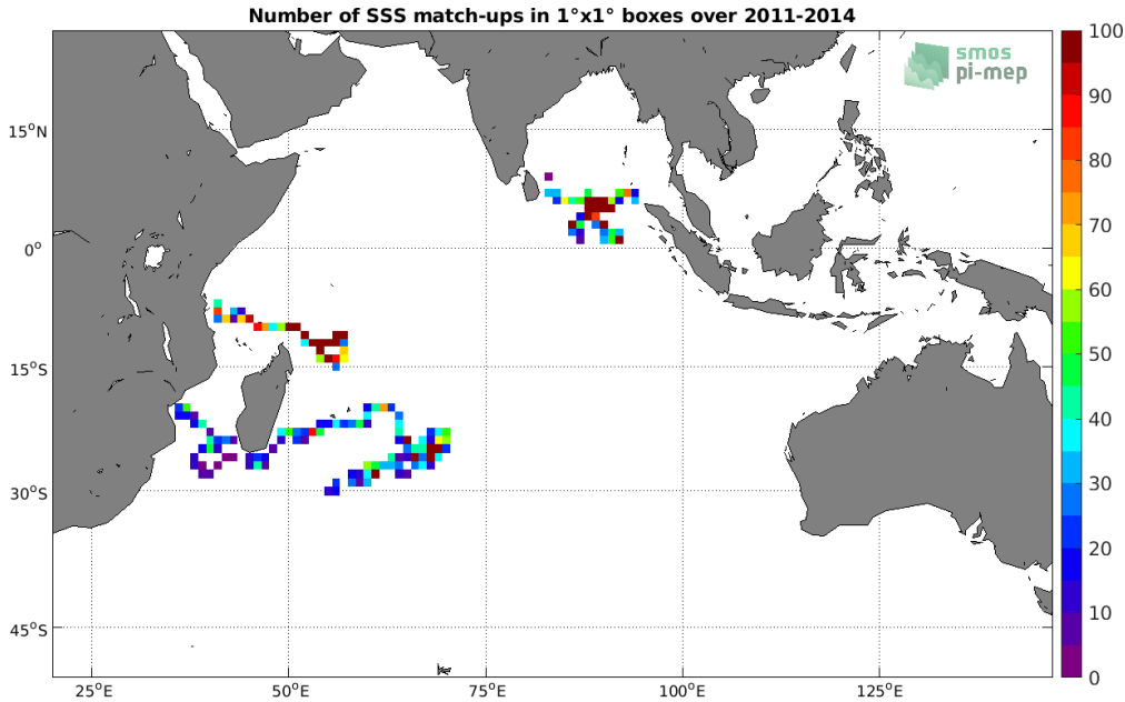
Figure 3: Number of SSS match-ups between Surface drifters SSS and the Aquarius SSS L4 OI v5 - Monthly (IPRC) SSS product for the Indian Ocean Pi-MEP region over 1^\circ \times 1^\circ boxes and for the full satellite product period.
