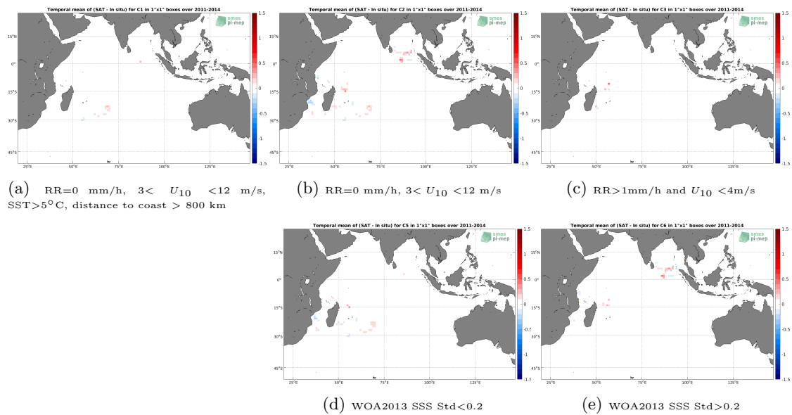
Figure 11: Temporal mean gridded over spatial boxes of size 1°x1° of \Delta SSS (Aquarius SSS L4 OI v5 - Monthly (IPRC) - Surface drifters) for 5 different subdatasets corresponding to:RR=0 mm/h, 3 < U_{10} < 12 m/s, SST>5°C, distance to coast > 800 km (a), RR=0 mm/h, 3 < U_{10} < 12 m/s (b), RR>1mm/h and U_{10} < 4 m/s (c), WOA2013 SSS Std<0.2 (d), WOA2013 SSS Std>0.2 (e).
